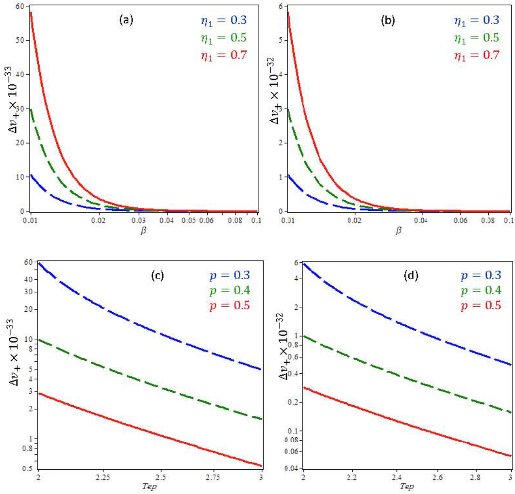
Figure 5.3 Effect on \Delta v_+ of \eta_1 ((a), (b)) with \beta taking remaining parameters q = 0.18, p = 0.3, T_{ip} = 2.5 and T_{ep} = 2 and p ((c), (d)) with T_{ep} taking as (a), \beta = 0.01 and \eta_1 = 0.3 in case of HRR (left column) and WRR (right column).
