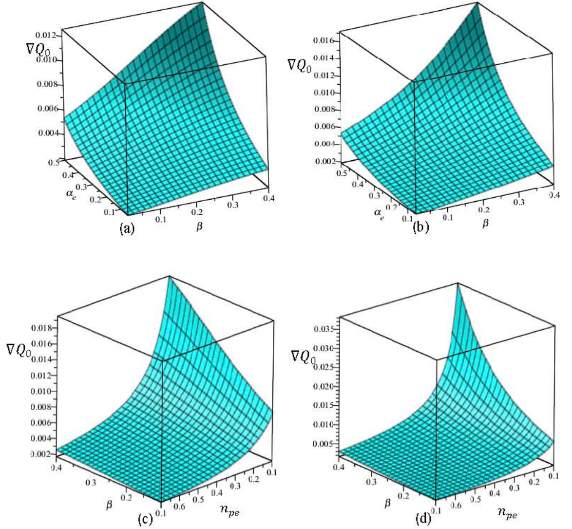
Figure 3.1 Effect of \alpha_e ((a) and (b)) taking T_{ie} = T_i/T_e = 0.001 , T_{ep} = T_e/T_p = 1 , \alpha_p = 0.5 , U_0 = 0.0075 , and \epsilon = 0.1 ; and n_{pe} = n_{p0}/n_{e0} ((c) and (d)) taking T_{ie} = 0.001 , T_{ep} = 1 , \alpha_{e,p} = 0.1 , U_0 = 0.0075 , and \epsilon = 0.1 along with relativistic streaming factor \beta = u_{i0}/c on the positive phase shift \nabla Q_0 for both of WRR (left column) and HRR (right column).
