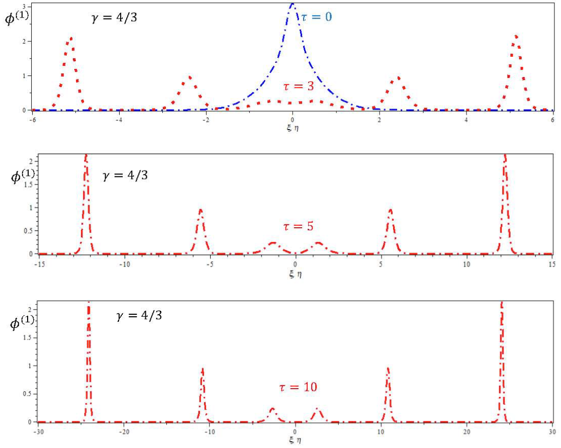
Figure 2.5 Electrostatic potential ( \phi^{(1)} ) profiles due to the interaction between equal amplitude triple solitons at different \tau for ultra-relativistic ( \gamma = 4/3 ) degenerate electrons and positrons, and inertial non-relativistic helium ions, where \eta_1 = 0.6 , \lambda = 0.10 , \beta = 0.10 , \mu = 0.40 , k_1 = 1 , k_2 = 2 , k_3 = 3 , and \sigma = 0.5 .
