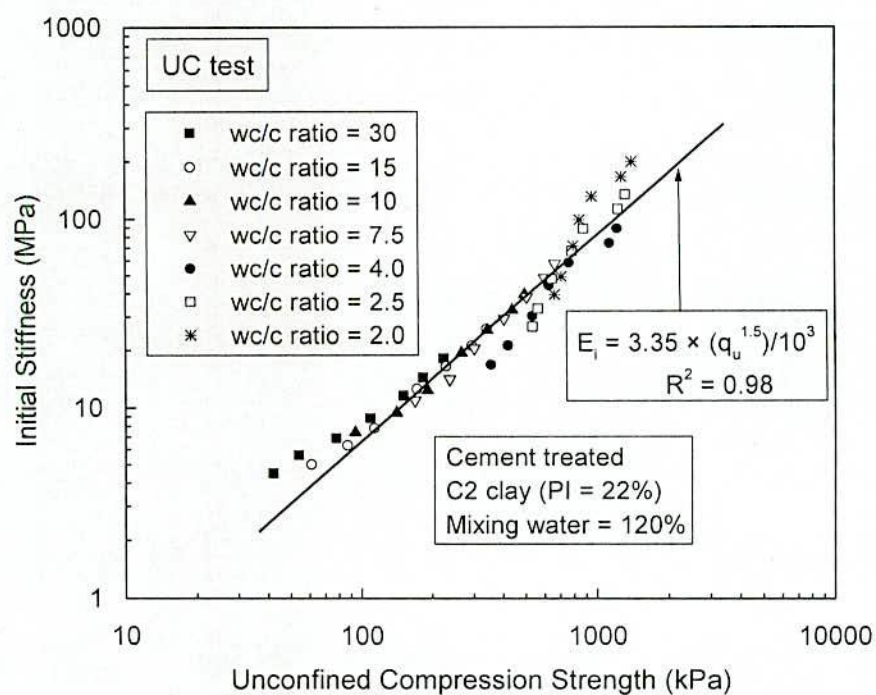
Fig. 5.56 Relationship between q_u and E_i Shown in Terms of wc/c Ratio of Cement Treated C2 clay
