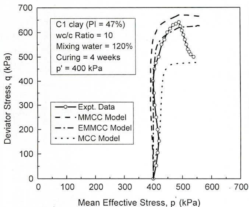
Fig. 6.37 Comparison of MCC, MMCC and EMMCC Predictions and Observed Undrained Stress Path in CIU for Cement Treated C1 clay ( w_c/c = 10 ) at p'_0 = 400 kPa
