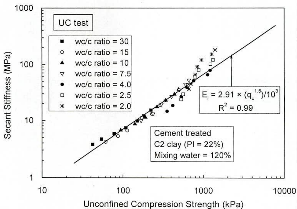
Fig. 5.61 Relationship between q_u and E_{50} Shown in Terms of wc/c Ratio of Cement Treated C2 clay
