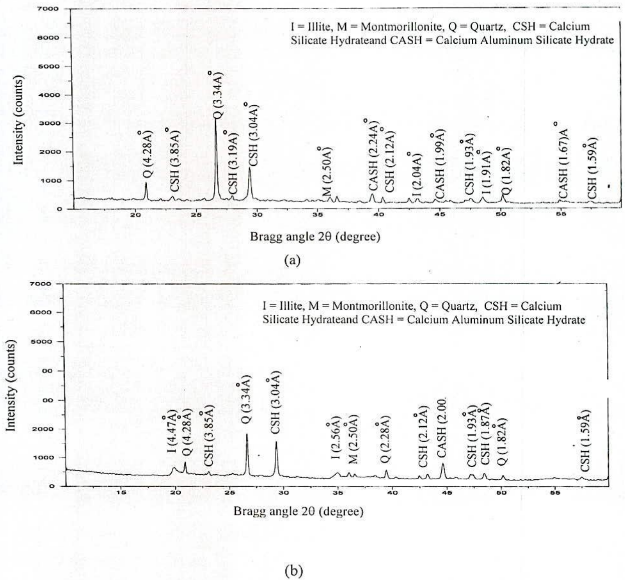
Fig. 4.11 X-Ray Diffraction Patterns at 4 weeks Curing time and 120% Mixing water of 30% Cement Treated Clays (a) C3 clay and (b) C1 clay
