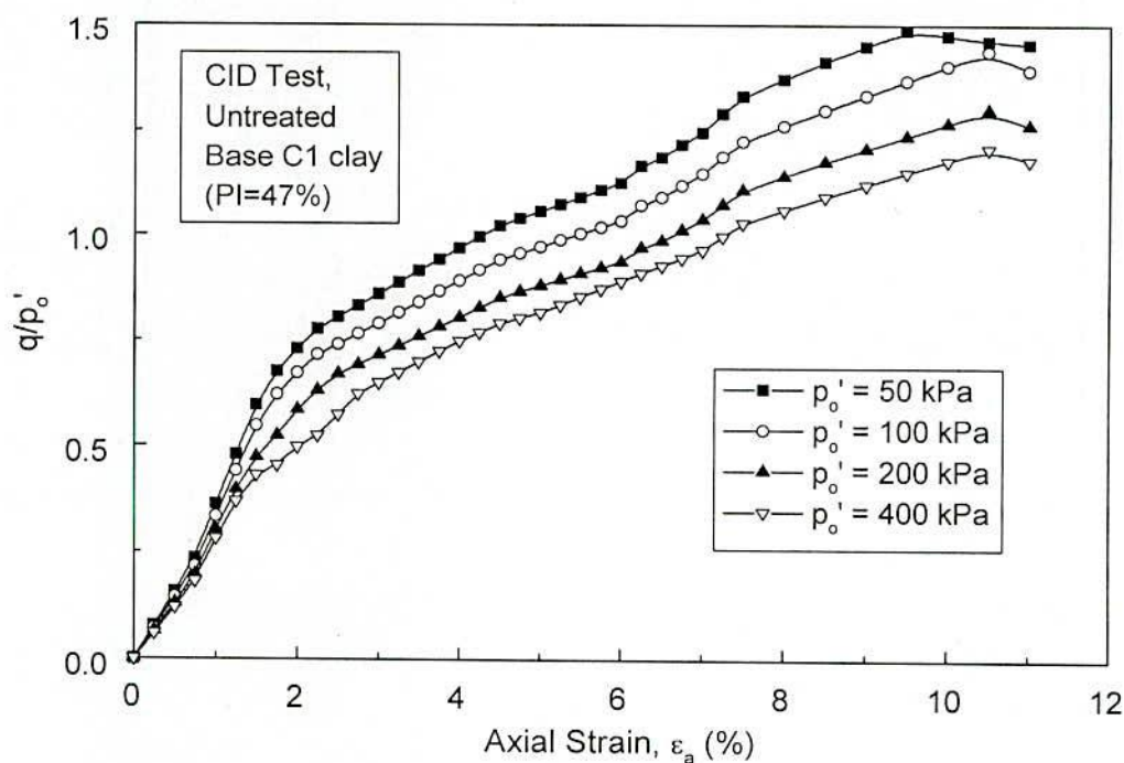
Fig. 5.106 Normalized Relationship Plots q/p'_o \cdot \epsilon_a for Untreated Base C1 Clay
