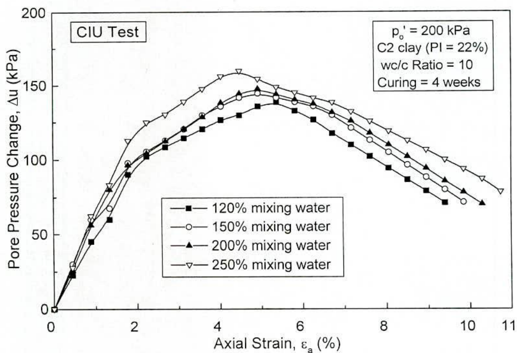
Fig. 5.91 Effect of Mixing Water Content on Pore Pressure Versus Axial Strain Response of C2 clay
