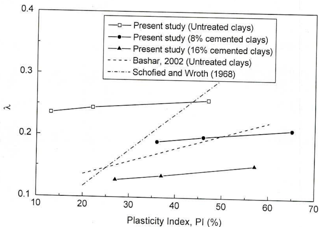
Fig. 6.12 Effect of Cement (curing = 4 w) on Correlation between Critical Compressibility Index ( \lambda ) and Plasticity Index (PI)
