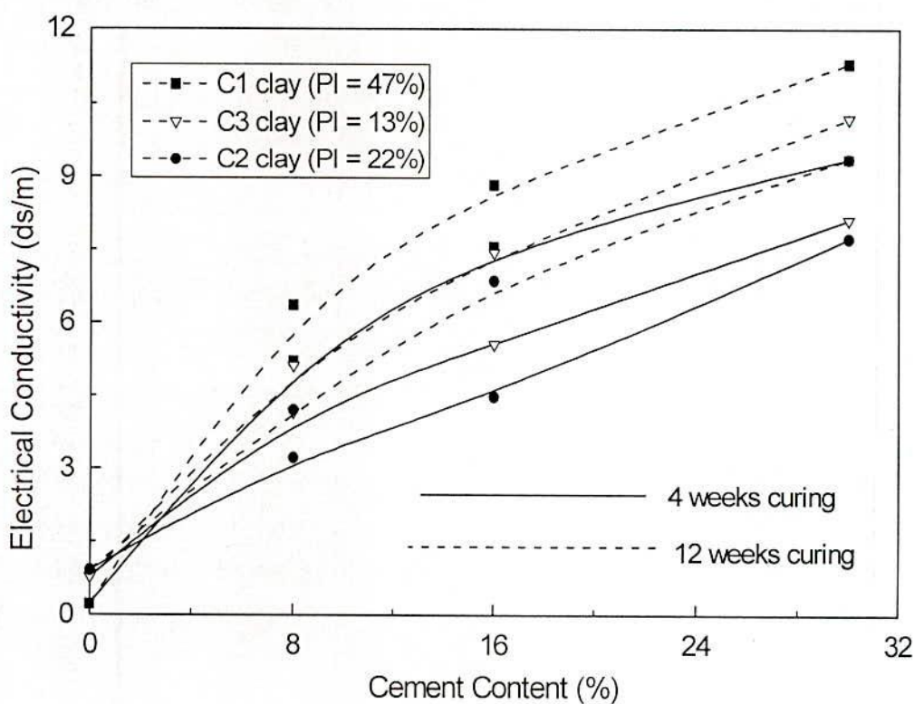
Fig. 4.6 Effect for Cement Content, Curing Time and Clay Type on Electrical Conductivity of Treated Soils (mixing water = 120%)
