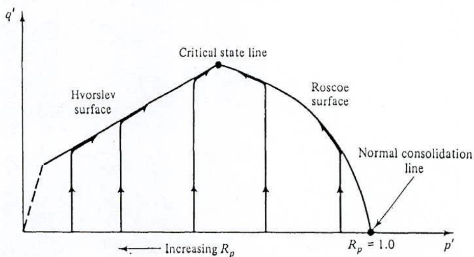
Fig. 2.53 Definitions of Hvorslev Surface, Roscoe Surface and Critical State Line (after Atkinson and Bransby, 1978)
