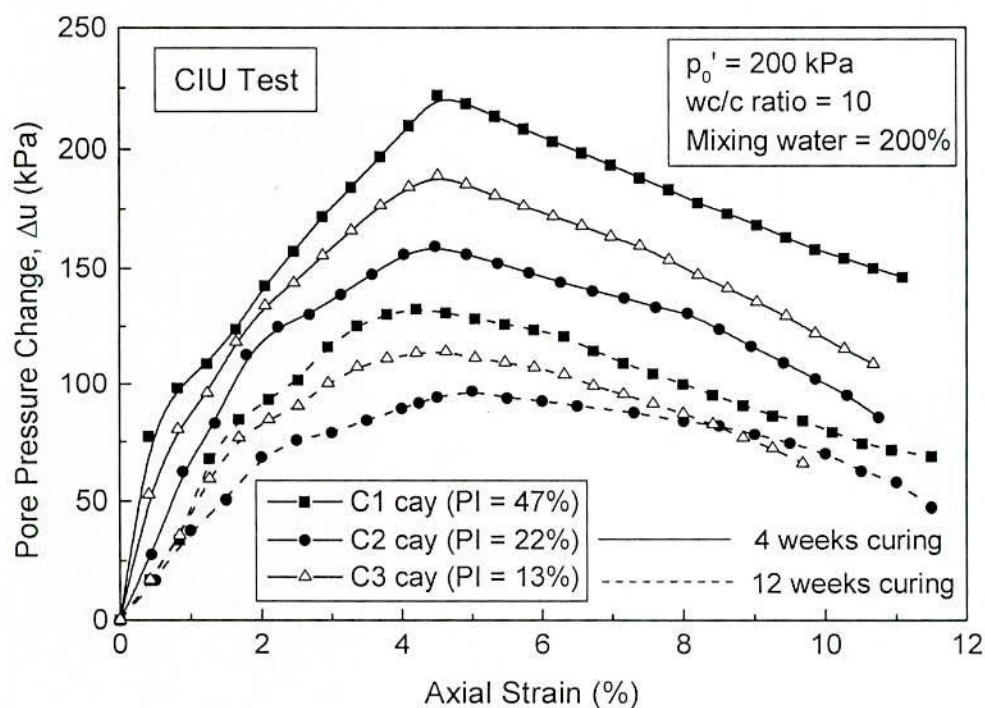
Fig. 5.90 Effect of Curing Time and Clay Type on Pore Pressure Versus Axial Strain Response
