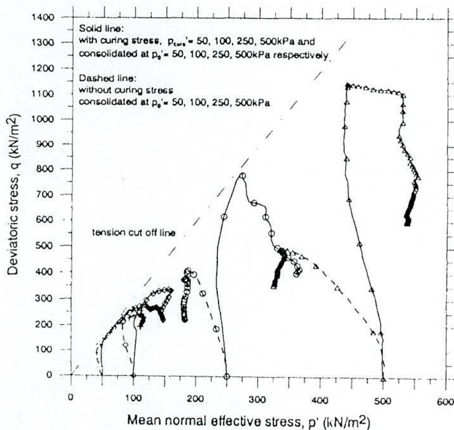
Fig. 2.39 Effect of Pre-Shear Consolidation Pressure on Undrained Stress Paths for Cement Treated and Untreated Clay (after Ghee et al., 2004)
