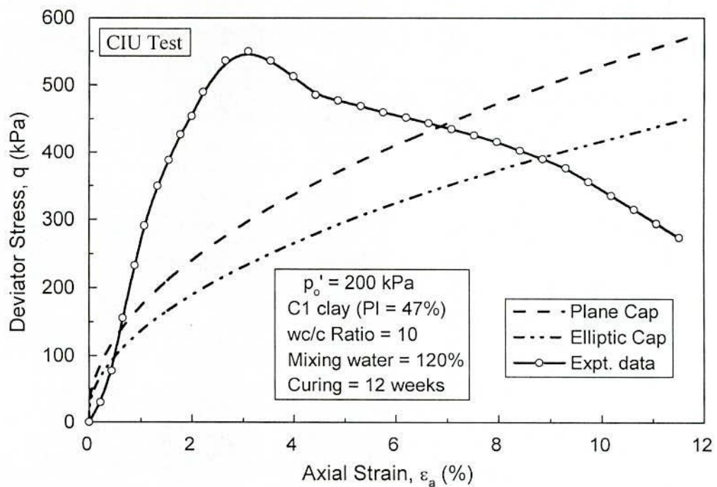
Fig. 6.46 Comparison of Plane Cap and Elliptic Cap Predictions and Observed Deviator Stress-Axial Strain Curves in CIU Test for Treated C1 clay at p'_0 = 200 kPa, w_c/c = 10 and Curing = 12 w
