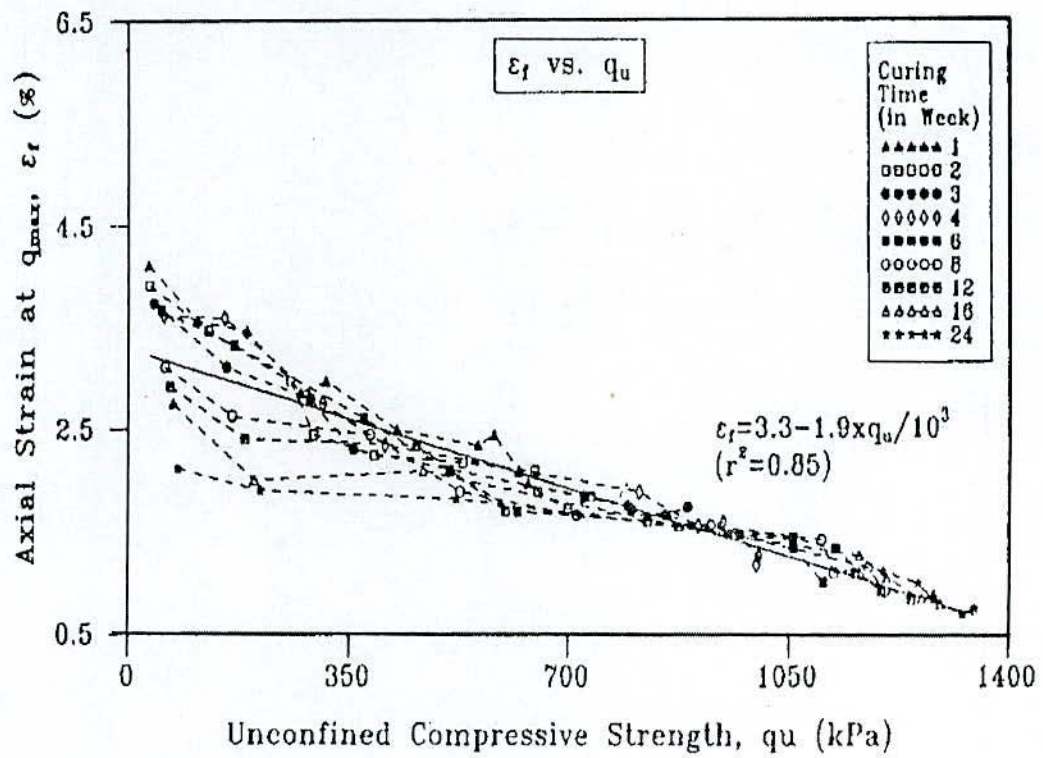
Fig. 2.42 Relationship between q_u and Axial Strain at q_{max} Shown in Terms of Curing Time for Cement Treated Clays (after Kamaluddin, 1995)
