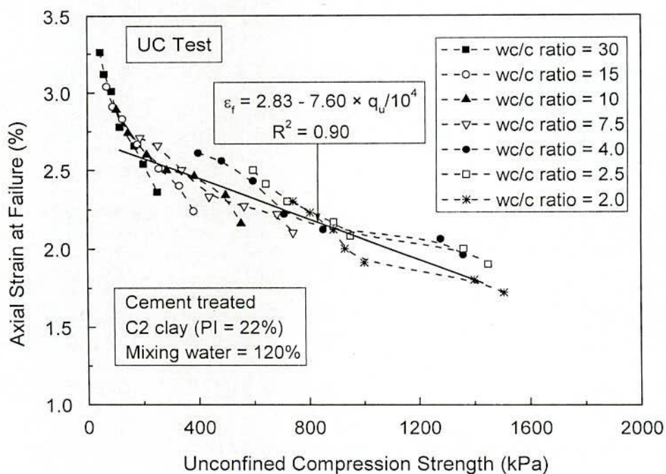
Fig. 5.51 Relationship between q_u and Axial Strain at Failure Shown in Terms of wc/c Ratio for Cement Treated C2 clay
