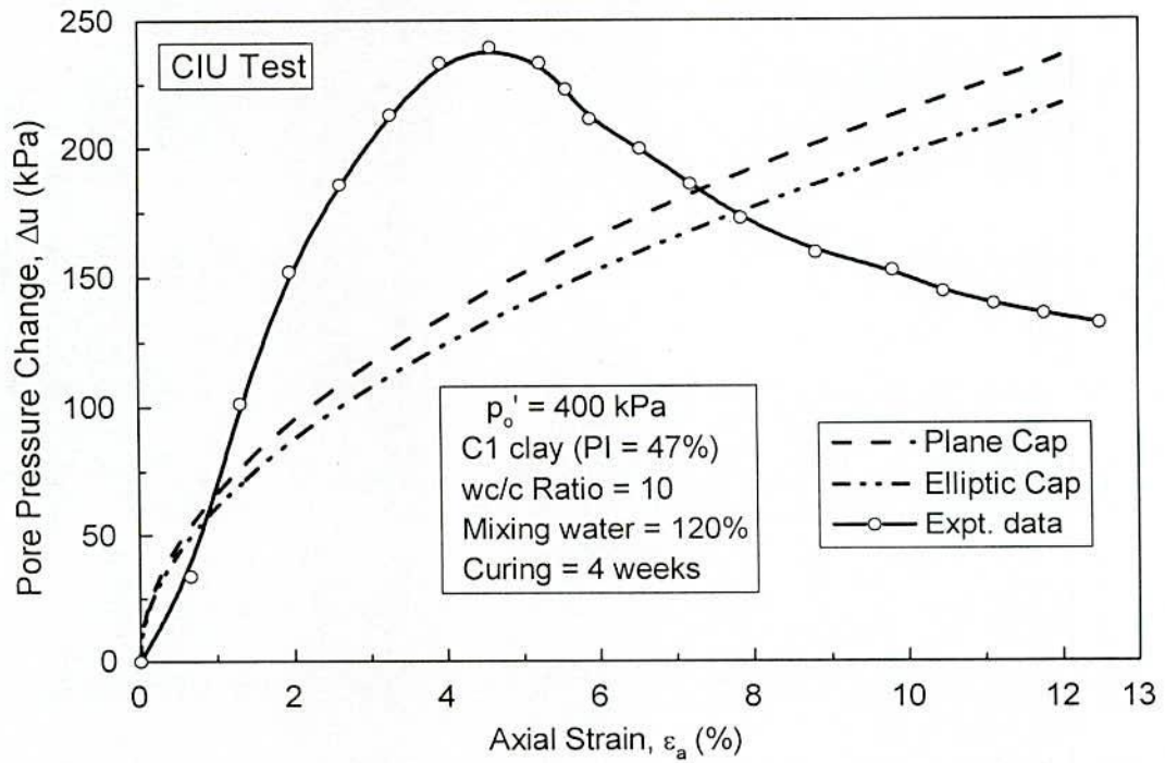
Fig. 6.48 Comparison of Plane Cap and Elliptic Cap Predictions and Observed Pore Pressure Change-Axial Strain Curves in CIU Test for Treated C1 clay at p_o' = 400 kPa, w/c = 10 and Curing = 4 w
