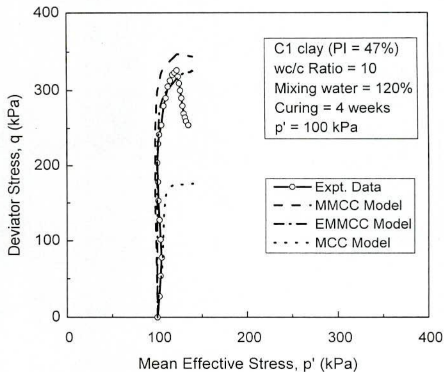
Fig. 6.35 Comparison of MCC, MMCC and EMMCC Prediction and Observed Undrained Stress Path in CIU for Cement Treated C1 clay ( w/c = 10 ) at p'_o = 100 kPa
