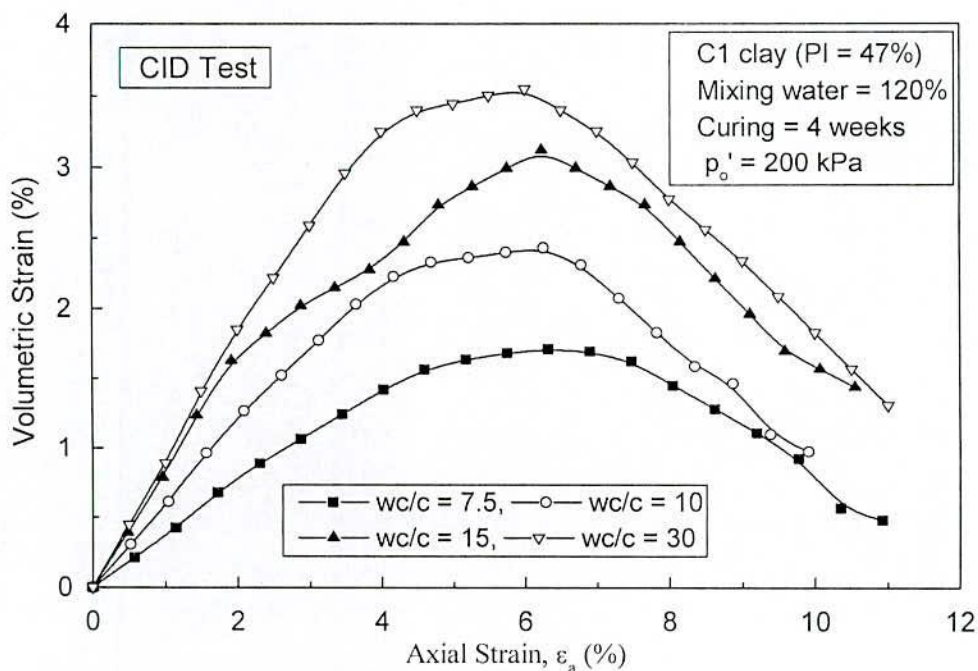
Fig. 5.110 Effect of Clay-Water/Cement ( wc/c ) Ratio on Volumetric Strain Versus Axial Strain Response of C1 Clay
