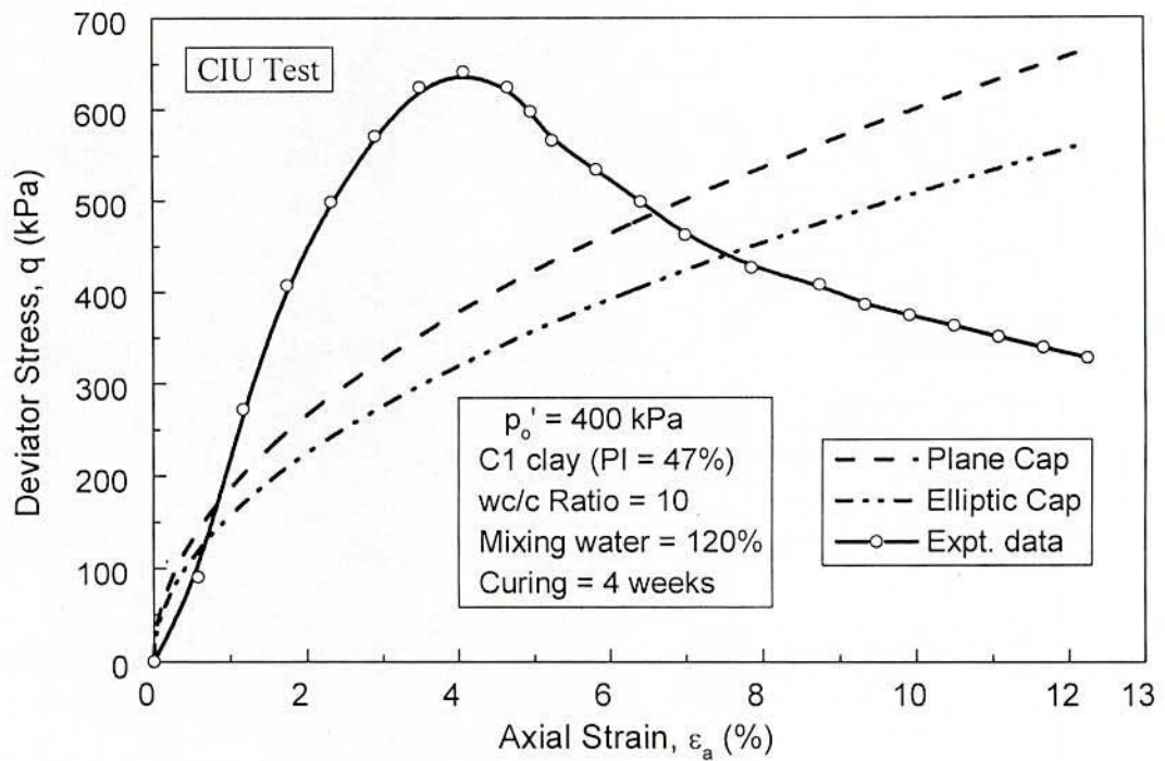
Fig. 6.45 Comparison of Plane Cap and Elliptic Cap Predictions and Observed Deviator Stress-Axial Strain Curves in CIU Test for Treated C1 clay p'_0 = 400 kPa, w_c/c = 10 and Curing = 4 w
