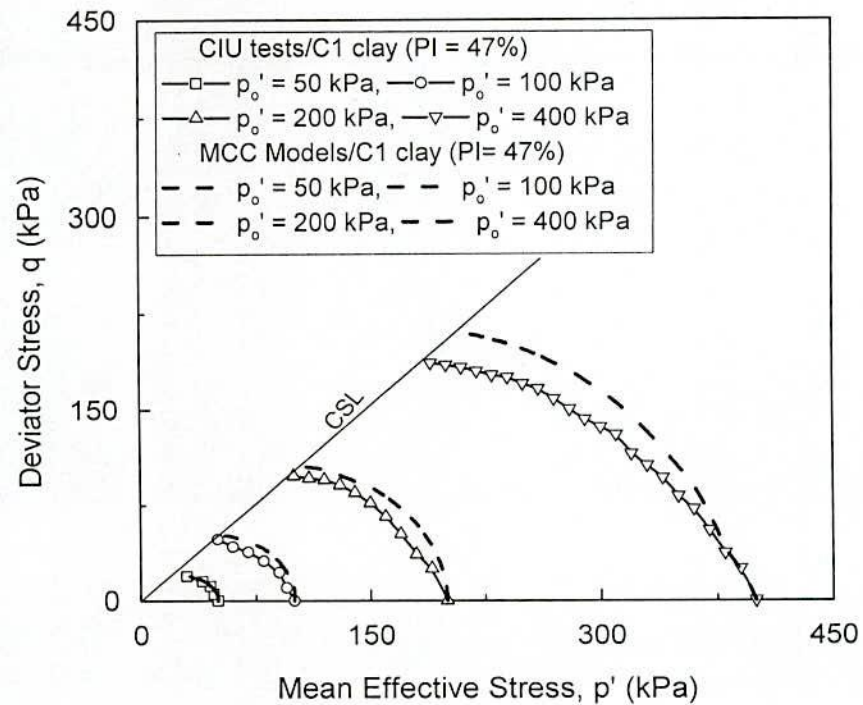
Fig. 6.34 Comparison of MCC Prediction and Observed Undrained Stress Path in CIU Test for Untreated Base C1 clay
