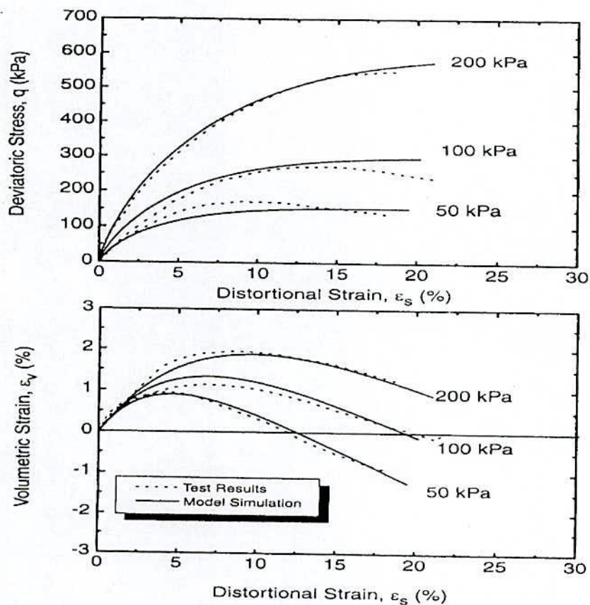
Fig. 2.55 Comparison of Constitutive Model prediction and Test results from Drained Test for Stabilized Soil (after Youwai and Bergado, 2003)
