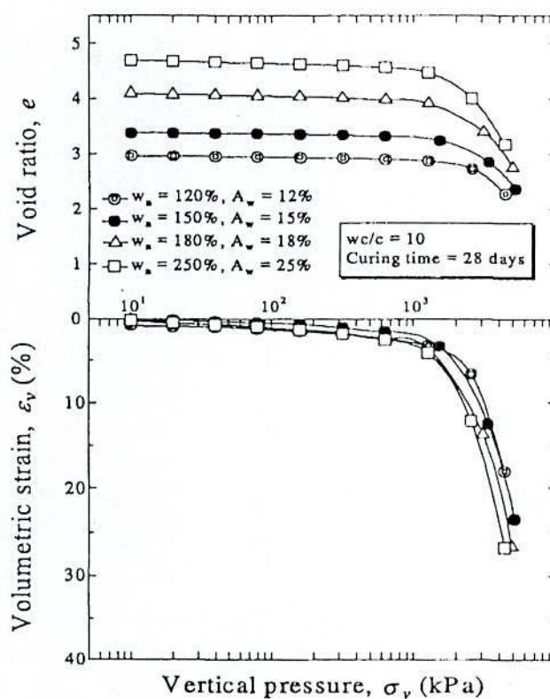
Fig. 2.28 e - \log \sigma'_v and \epsilon_v - \log \sigma'_v Relationships of Cement Treated Ariake Clay with same w_c/c Ratio, 10 (after Miura et al., 2001)
