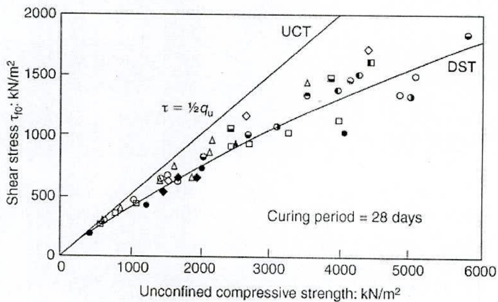
Fig. 2.51 Relation between DS and UC Test Results for Cement Treated Clays (after Porbaha et al., 2000)
