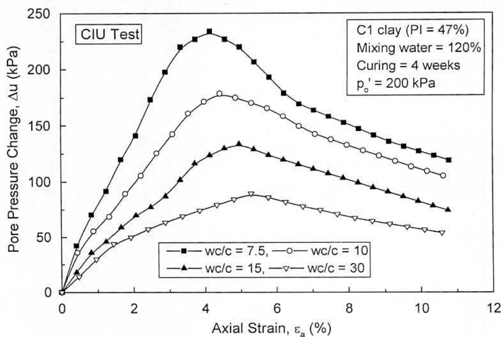
Fig. 5.89 Effect of Clay-Water/Cement ( wc/c ) Ratio on Pore Pressure Versus Axial Strain Response of C1 Clay
