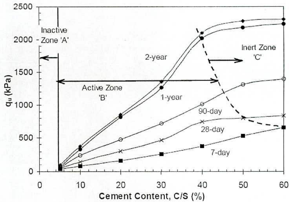
Fig. 2.7 Unconfined Compressive Strength and Cement Content Relationship (120% water) at different Curing Periods for Cement Treated clays (after Kamruzzaman et al., 2004)
