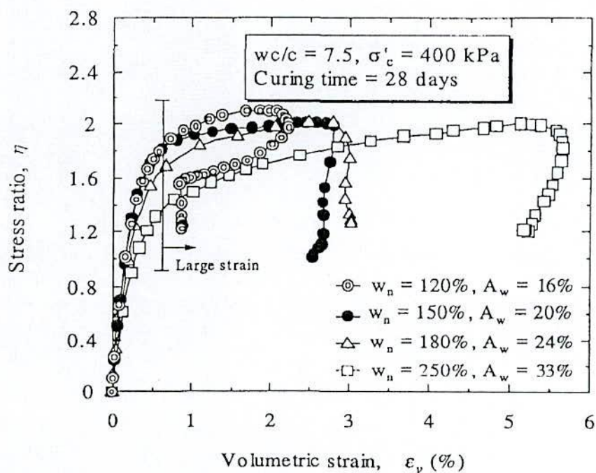
Fig. 2.38 Effect of Mixing Water Content on (\eta, \epsilon_v) Relationships for w/c Ratio = 7.5 and p'_0 = 400 \text{ kPa} for Cement Treated Clays (after Miura et al., 2001)
