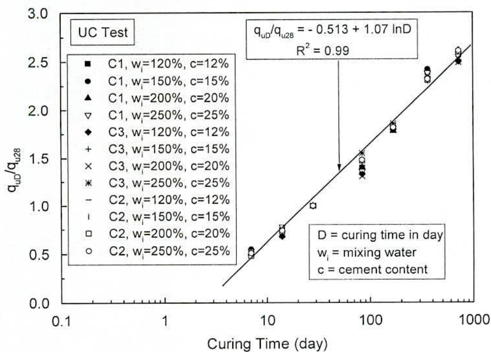
Fig. 5.47 Strength Development with Time and its Generalization of Clays Studied
