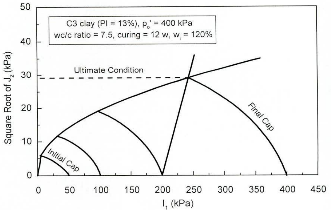
Fig. 6.50 Stress Path in I_1 - \sqrt{J_2} Space from Cap Model for Cement Treated (a) C1 clay and (b) C3 clay
