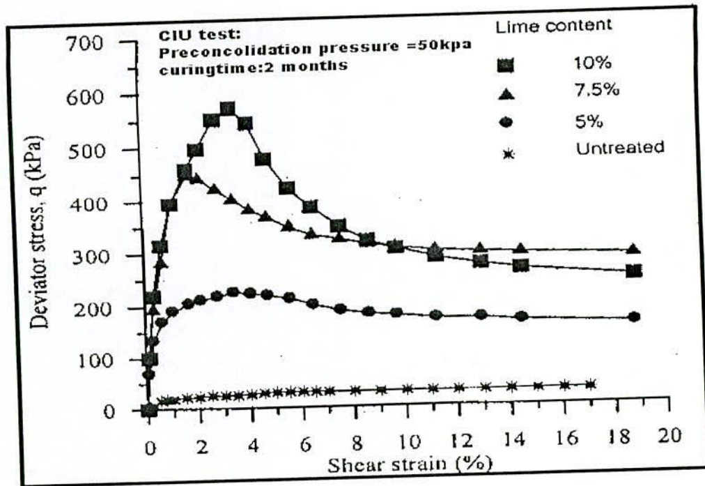
Fig. 2.34 Effect of Lime Content on (q-\epsilon_s) Relationships for Lime Treated Clays (after Bergado et al., 2003)
