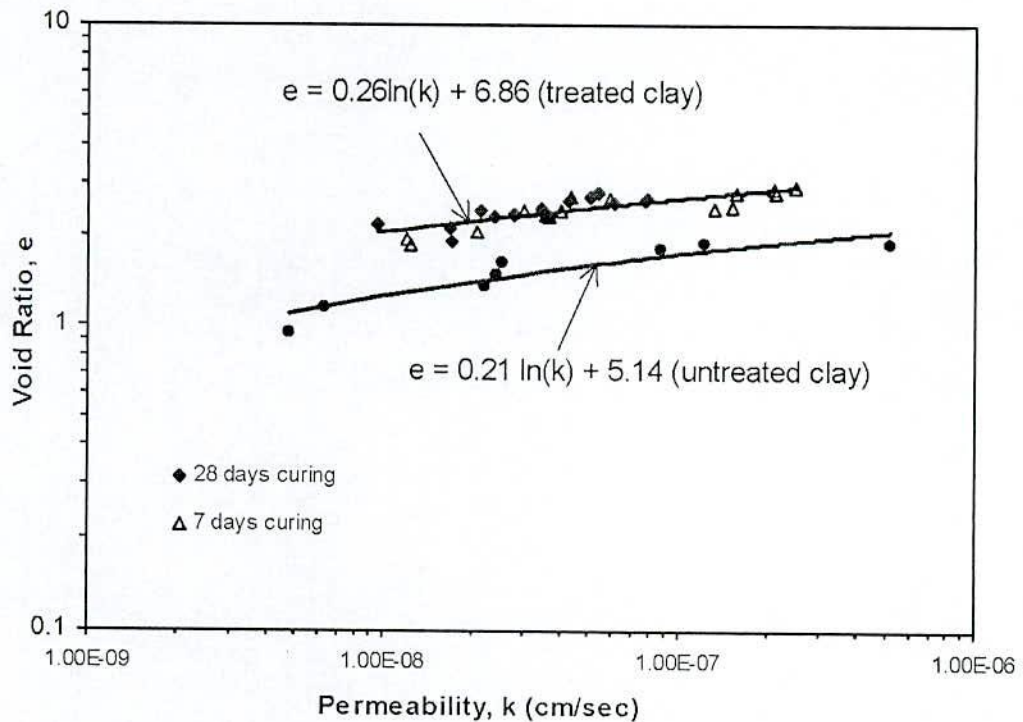
Fig. 2.33 Void ratio and Permeability (log-log) Relationships of Cement Treated Singapore Clays at w_i , 120% (after Chew et al., 2004)
