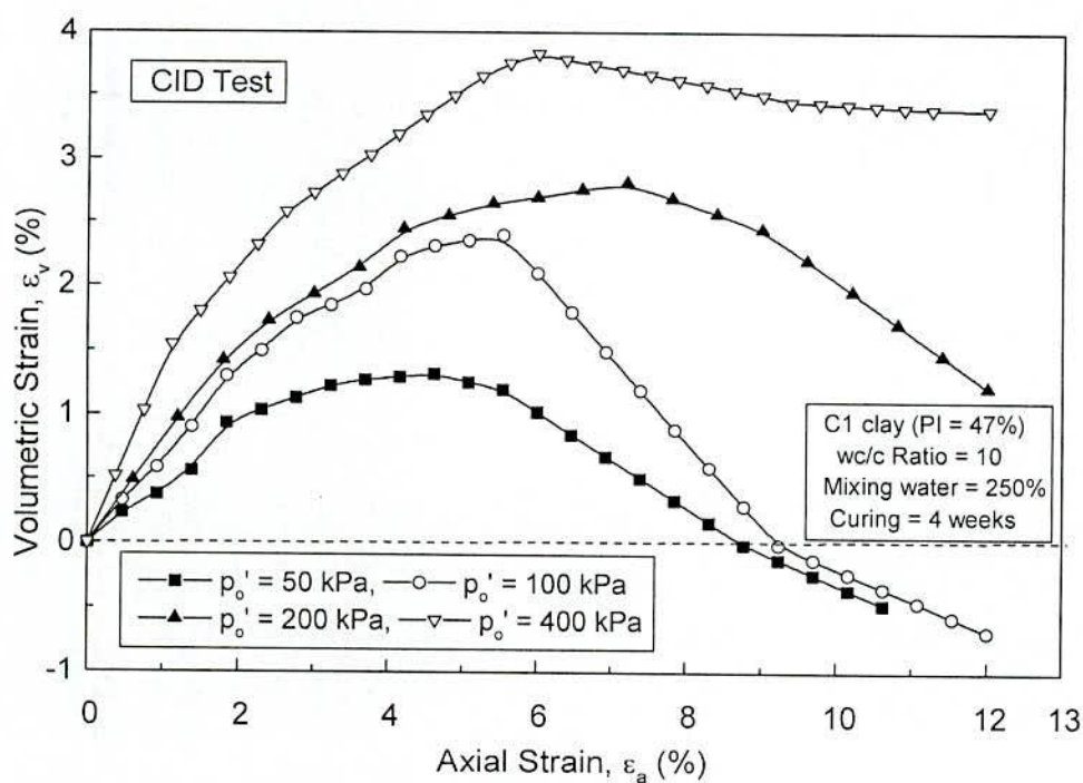
Fig. 5.113 Effect of Pre-Shear Effective Consolidation Pressure on Volumetric Strain Versus Axial Strain Response of C1 Clay
