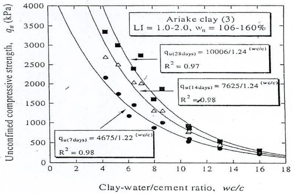
Fig. 2.49 Influence of wc/c on the Strength Development of Cement Admixed Ariake Clay (3) with its Various Fabric Pattern (after Horpibulsuk et al. 2000)
