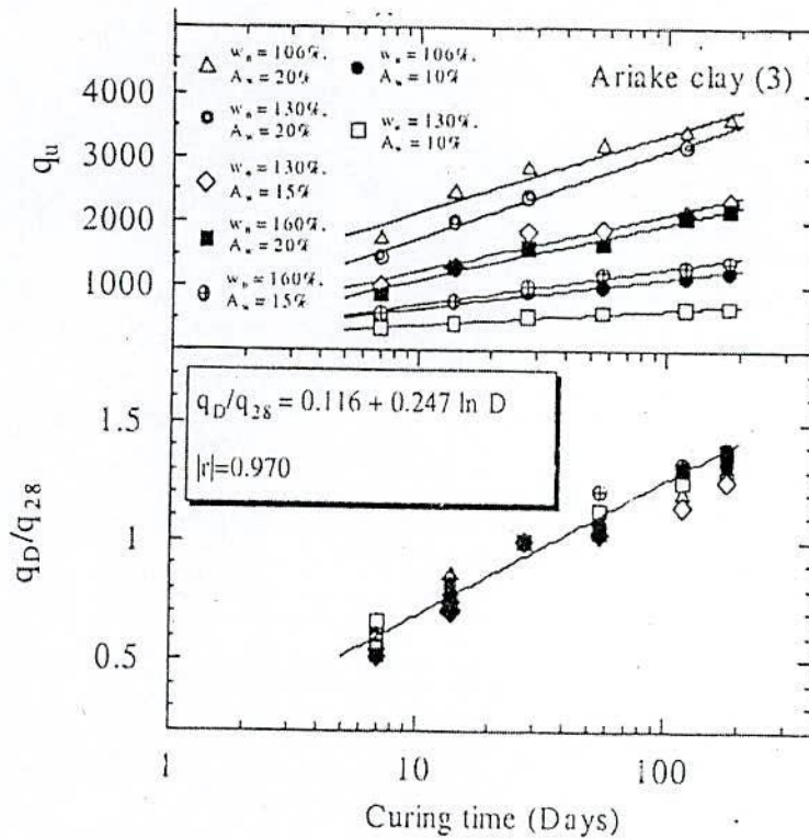
Fig. 2.50 Strength Development with Time and its Generalization of Cement Admixed Ariake Clay (3) (after Horpibulsuk et al. 2000)
