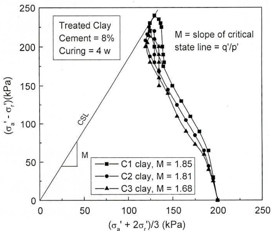
Fig. 6.5 Effective Stress Path for Three Cement Treated Clays at Cement = 8% and Water = 120%
