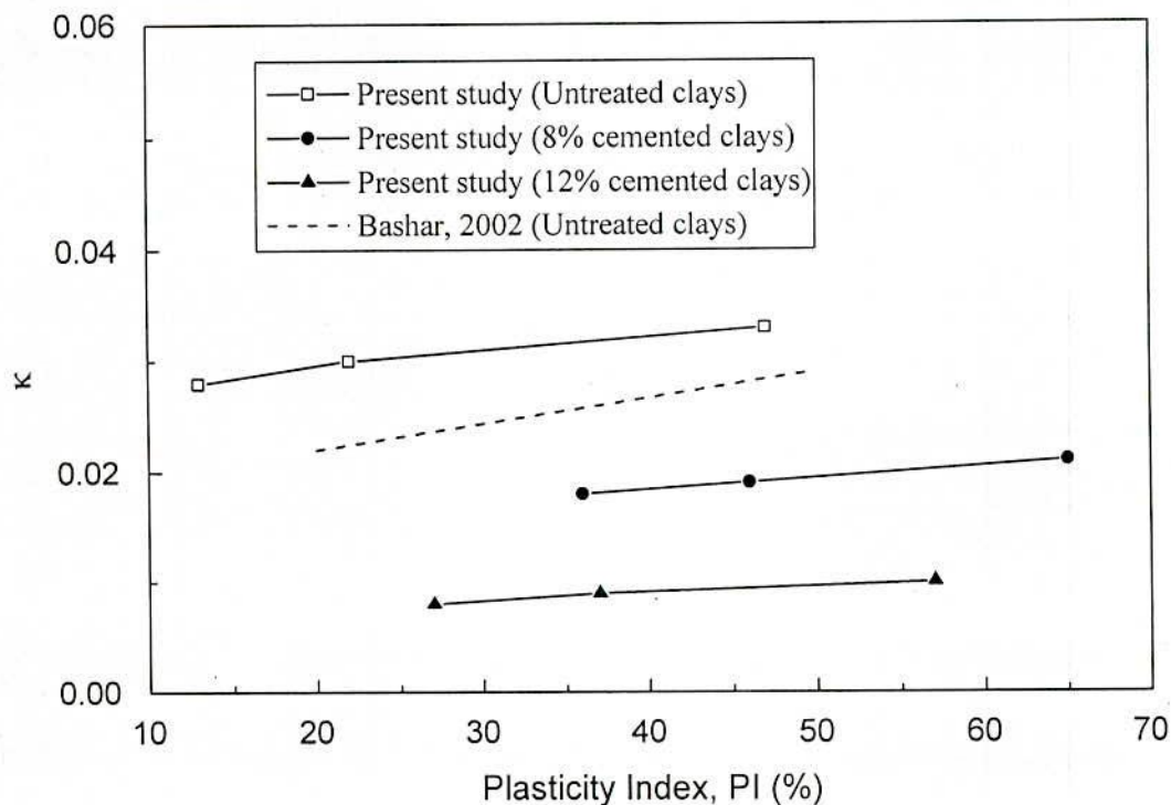
Fig. 6.14 Effect of Cement (curing = 4 w) on Correlation between Critical Swelling Index ( \kappa ) and Plasticity Index (PI)
