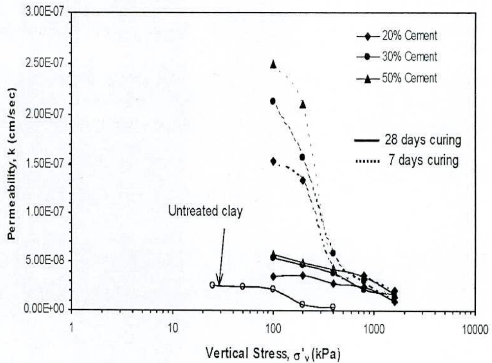
Fig. 2.32 Effect of Cement and Curing Time on k - \log \sigma'_v Relationships of Treated Singapore Marine Clays at w_i , 120% (after Chew et. al., 2004)
