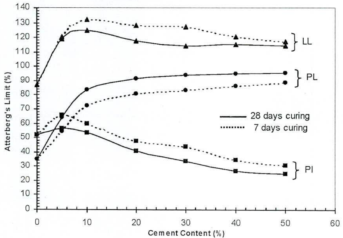
Fig. 2.27 Effect of Cement Content and Curing Time on Atterberg Limit for Cement Treated Clays (after Chew et al., 2004)
