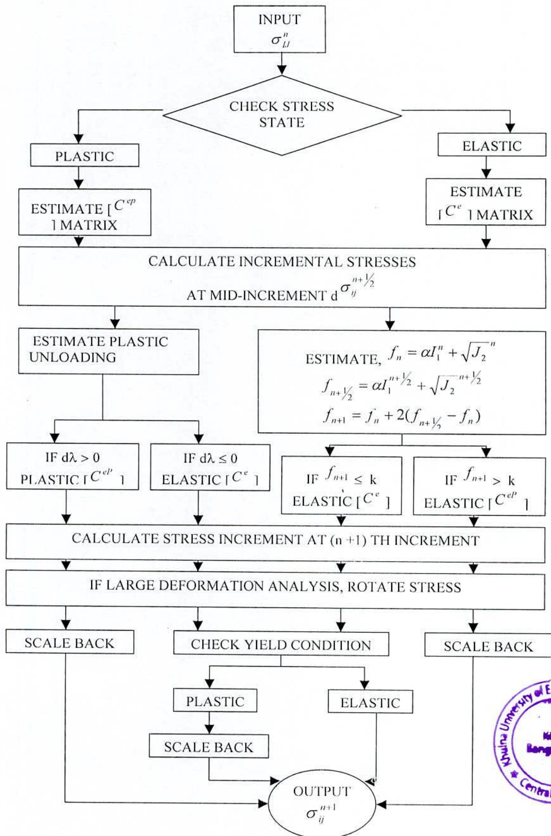
Fig. 2.61 Flow Chart for the Implementation of Coulomb and Prager Models in Cap Model (after Chen and Mizuno, 1990)
