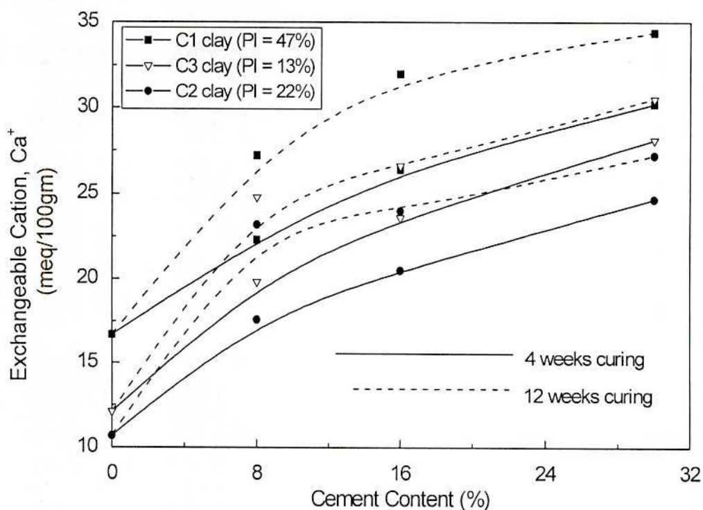
Fig. 4.8 Effect for Cement Content, Curing Time and Clay Type on Exchangeable Cation ( \text{Ca}^{2+} ) of Treated Soils (water = 120%)
