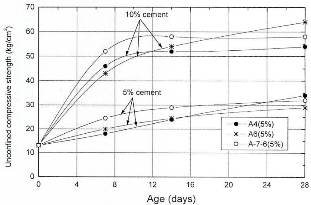
Fig. 2.8 Effect of Curing Age on Unconfined Compressive Strength for Soil-Cement Mix Specimens of Three Soils in Bangladesh (after Serajuddin and Azmal, 1991)
