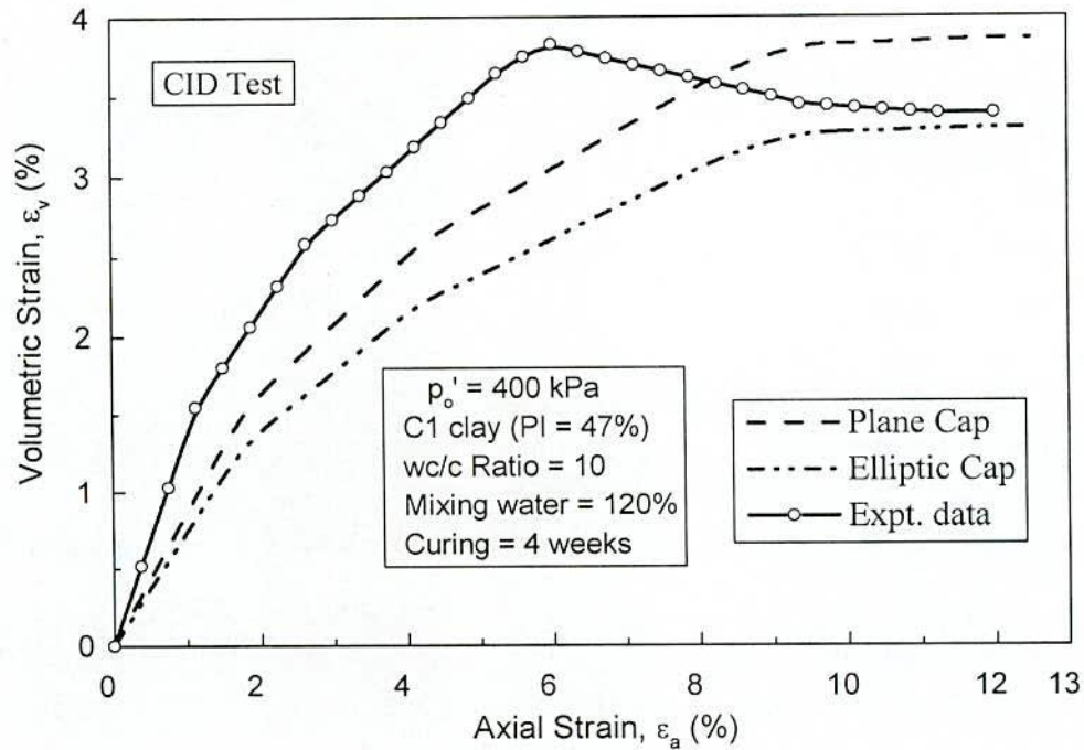
Fig. 6.42 Comparison of Plane Cap and Elliptic Cap Predictions and Observed Volumetric Strain-Axial Strain Curves in CID Test for Treated C1 clay at p'_0 = 400 kPa, w_c/c = 10 and Curing = 4 w
