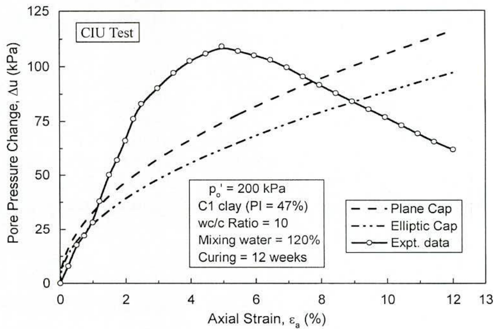
Fig. 6.49 Comparison of Plane Cap and Elliptic Cap Predictions and Observed Pore Pressure Change-Axial Strain Curves in CIU Test for Treated C1 clay at p_o' = 200 kPa, w/c = 10 and Curing = 12 w
