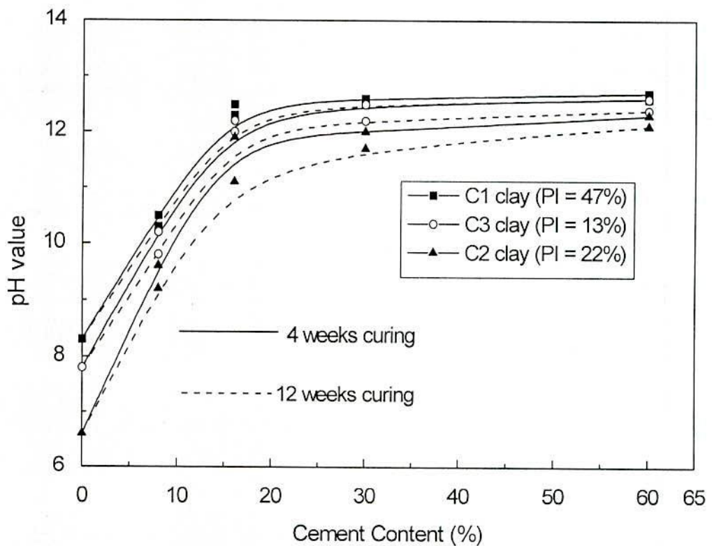
Fig. 4.2 Effect of Cement Content, Curing Time and Clay Type on pH value for Cement Treated Clays (mixing water = 120%)
