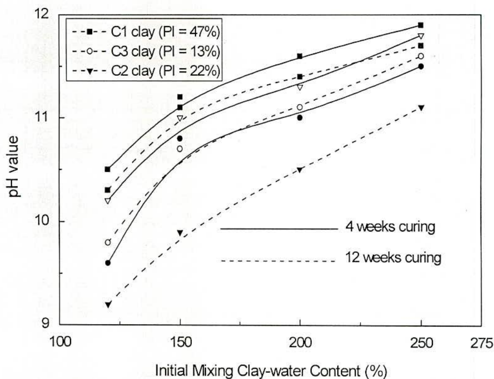
Fig. 4.3 Effect of mixing Water Content, Curing Time and Clay Type on pH value for Cement Treated Clays (wc/c ratio = 15)
