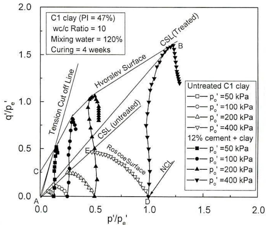
Fig. 6.11 Paths in q'/p_e' : p'/p_e' Space of Untreated and Cement Treated C1 clay
