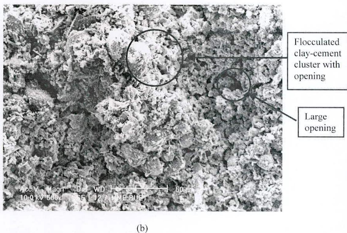
Fig. 4.17 SEM Image of 30% Cement Treated Clays (a) C1 clay and (b) C3 clay (4 weeks curing time and 120% mixing water)
