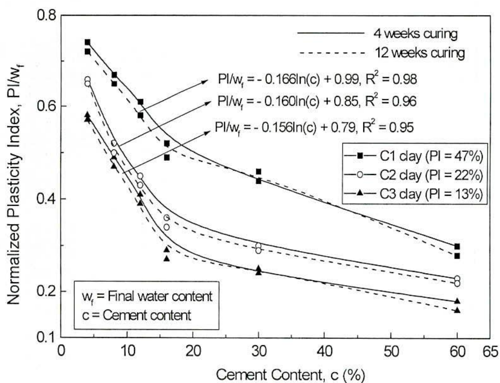
Fig. 4.33 Normalized Plasticity Index of Cement Treated clays (mixing water = 120%)
