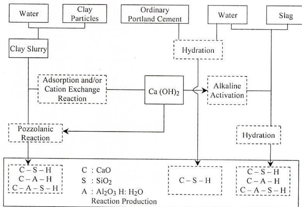
Fig. 2.2 Chemical Reaction between Soil and Hardening Agents (after Saitoh et al., 1985)
