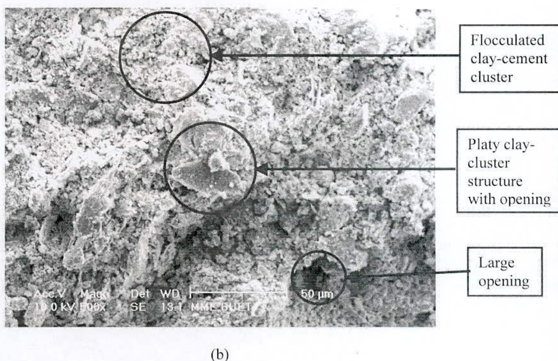
Fig. 4.16 SEM Image of 16% Cement Treated Clays (a) C1 clay and (b) C3 clay (4 weeks curing time and 120% mixing water)
