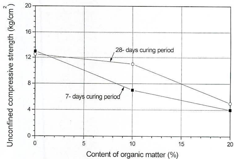
Fig. 2.22 Effects of Organic Matter on the Strength for Lime Treated Clays (after Arman and Muhfakh, 1972)
