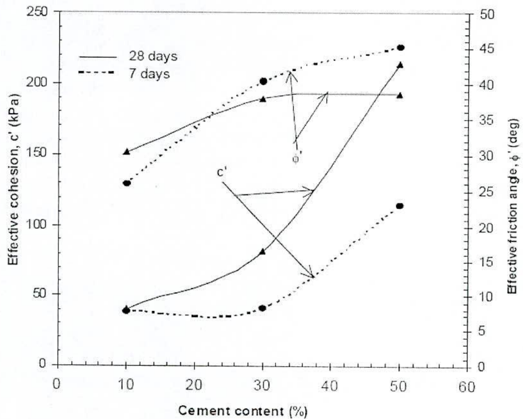
Fig. 2.41 Effect of Cement and Curing Time on Effective Shear Strength Parameters for Cement Treated Clays (after Kamruzzaman et al., 2004)
