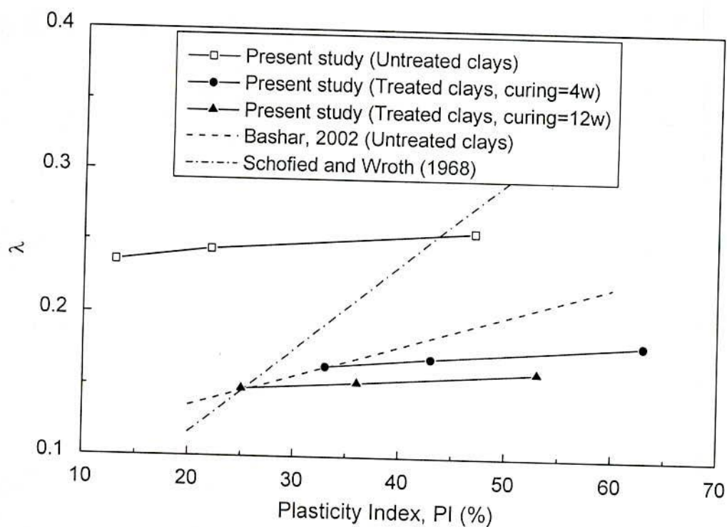
Fig. 6.13 Effect of Curing Time (cement = 12%) on Correlation between Critical Compressibility Index ( \lambda ) and Plasticity Index (PI)
