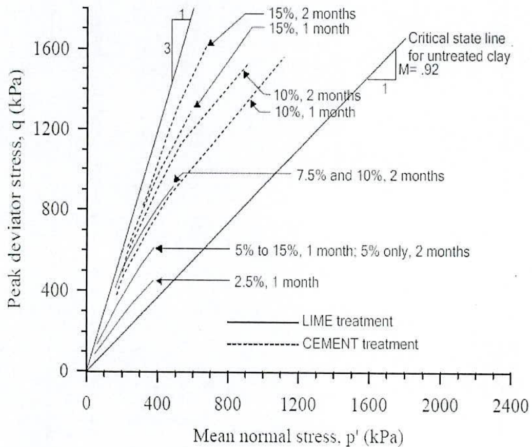
Fig. 2.37 q_{\max} - p' Relationships for Cement Treated Clays from CIU Tests (after Bergado et al., 2003)
