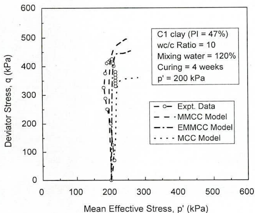
Fig. 6.36 Comparison of MCC, MMCC and EMMCC Prediction and Observed Undrained Stress Path in CIU for Cement Treated C1 clay ( w_c/c = 10 ) at p'_0 = 200 kPa
