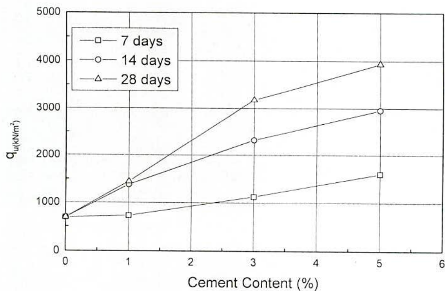
Fig. 2.6 Effect of Cement Content on Unconfined Compressive Strength for Coastal Soil of Bangladesh (after Siddique and Rajbongshi, 2002)
