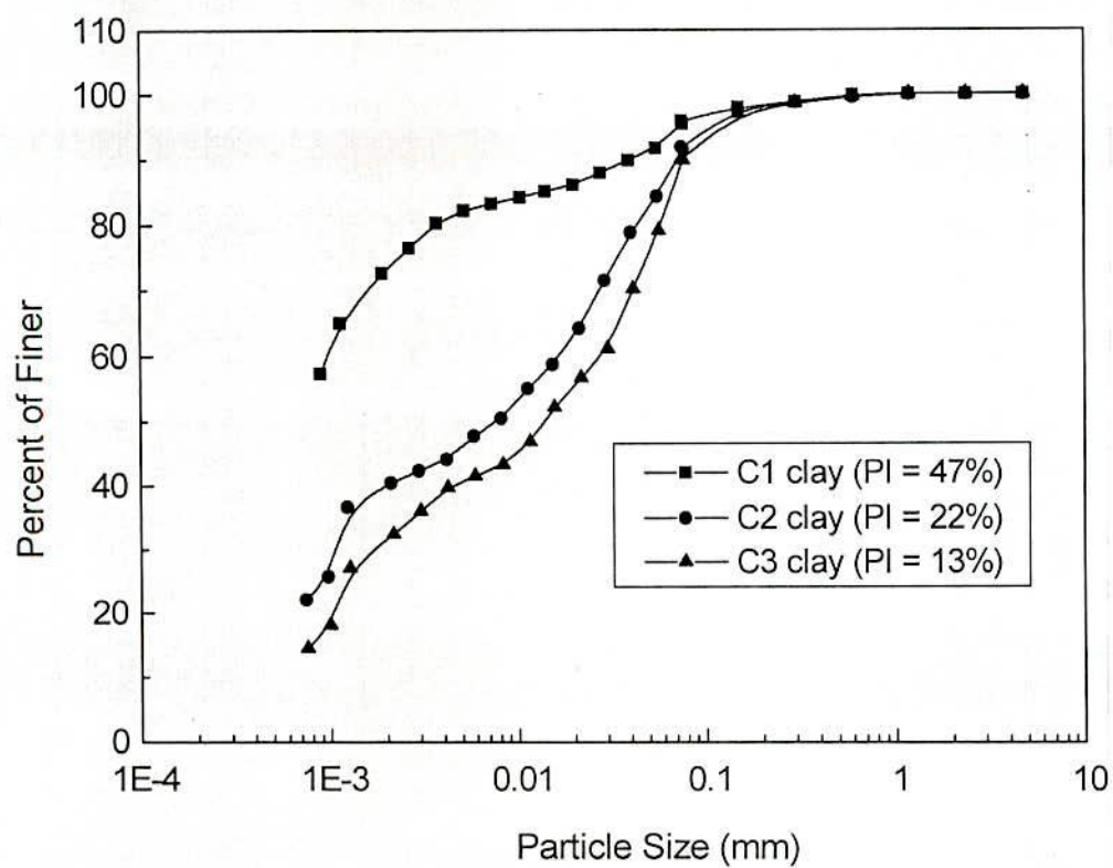
Fig. 4.20 Comparison of Grain Size Distribution Curve of Untreated Base Clays
