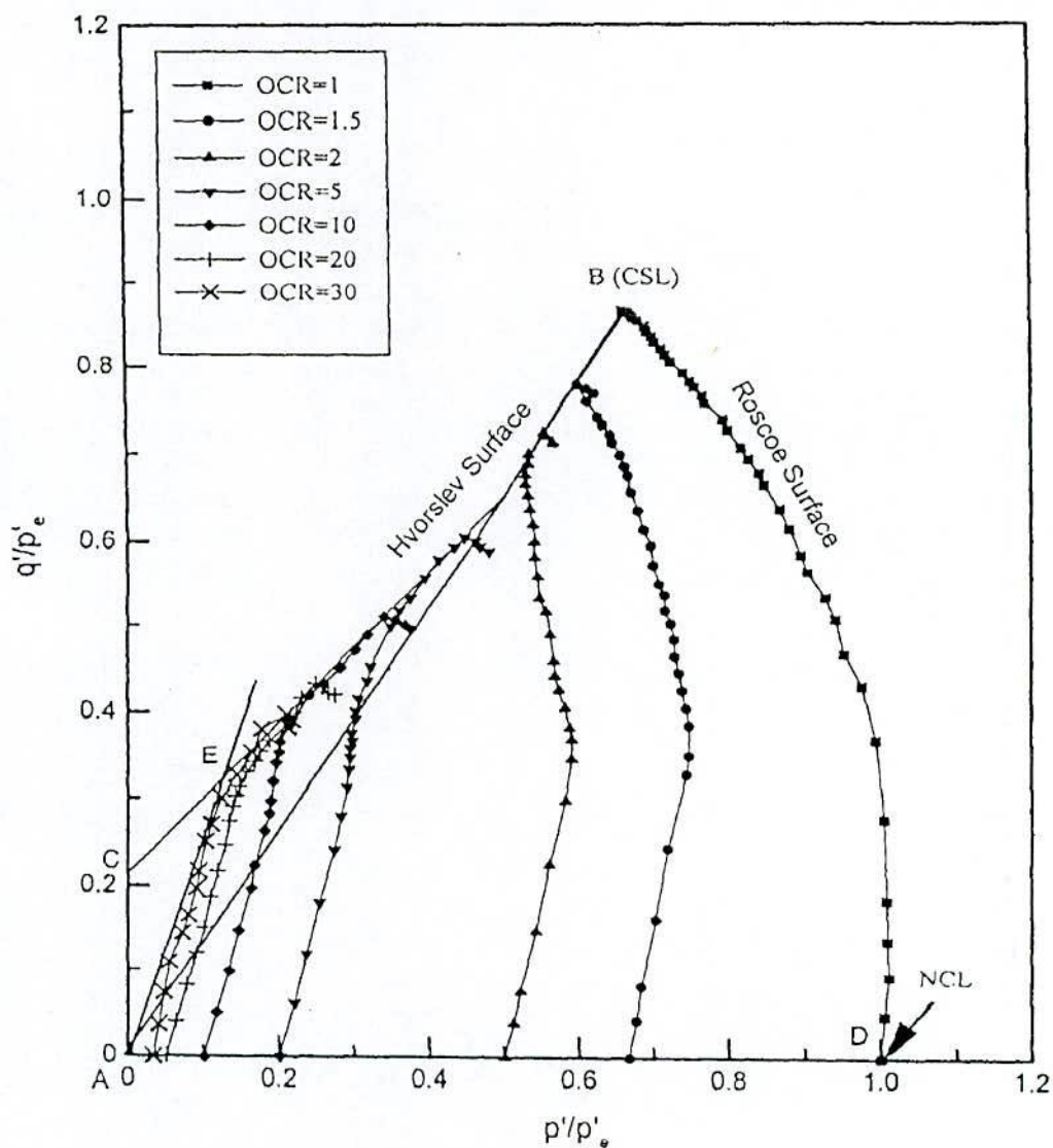
Fig. 2.54 Stress Paths, Roscoe Surface and Hvorslev Surface for Undained Tests on Coastal Soil in Bangladesh (Siddique et al., 2003)
