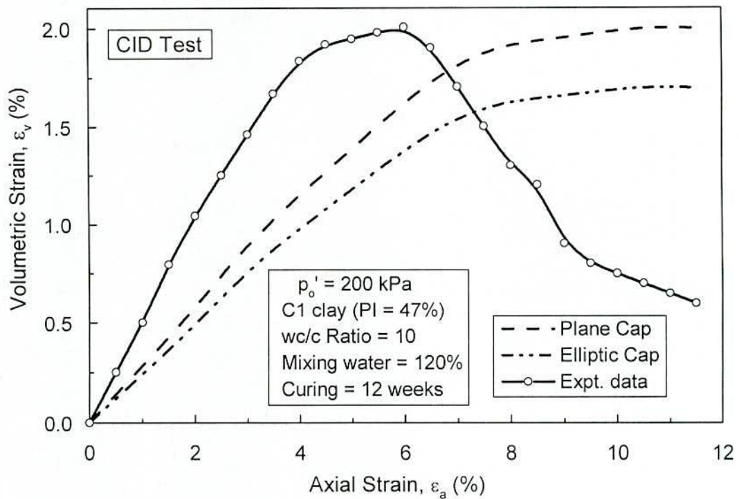
Fig. 6.43 Comparison of Plane Cap and Elliptic Cap Predictions and Observed Volumetric Strain-Axial Strain Curves in CID Test for Treated C1 clay at p'_0 = 200 kPa, w_c/c = 10 and Curing = 12 w
