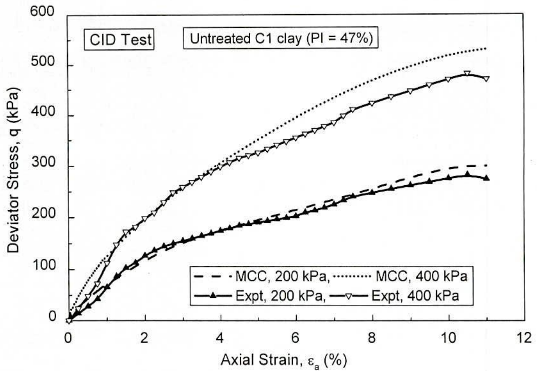
Fig. 6.18 Comparison of MCC Prediction and Observed Deviator Stress-Axial Curves in CID Test for Untreated Base C1 clay
