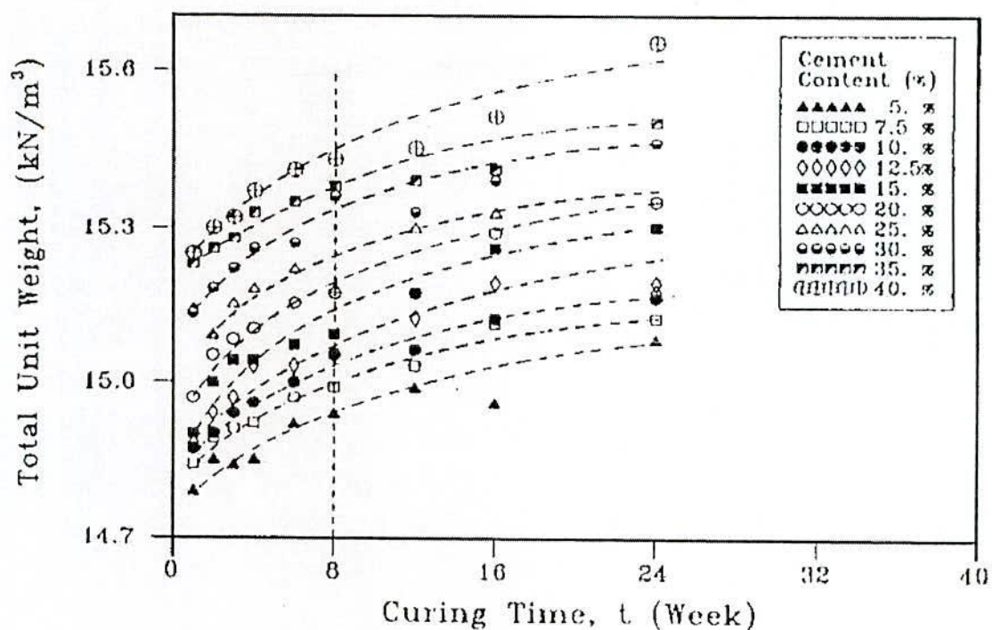
Fig. 2.25 Effect of Cement Content and Curing Time on Total Unit Weight for Cement Treated Clays (after Kamaluddin, 1995)
