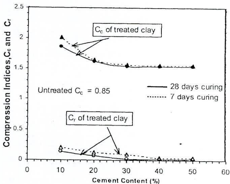
Fig. 2.29 Effect of Cement Content and Curing Time on Compression Indices of Cemented Singapore Clay with 120% water (after Chew et al., 2001)
