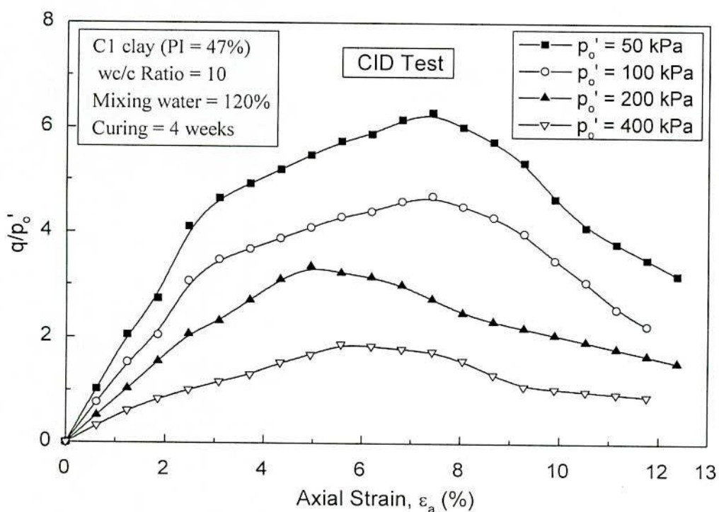
Fig. 5.107 Normalized Relationship Plots q/p'_o \cdot \epsilon_a for Cement Treated C1 clay
