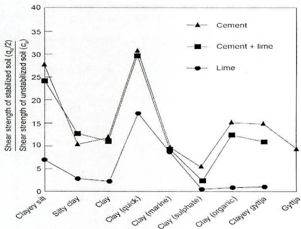
Fig. 2.9 Effect of Stabilizing Agents and Type of Clay on Unconfined Strength for Cement Treated clays (after Ahnberg et al., 1995)
