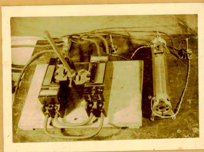
Fig 21 (b) Make-break mechanism, voltage divider and shunt
