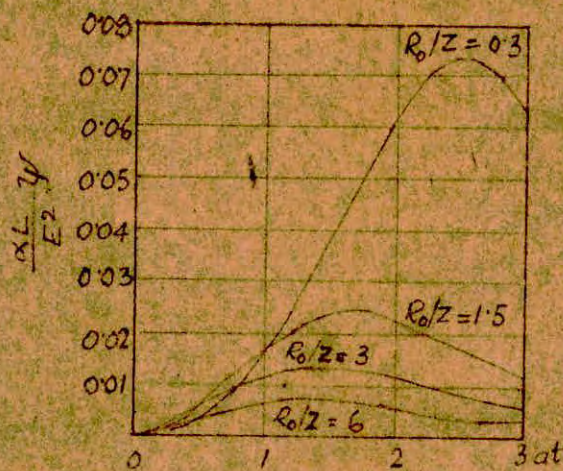
Fig 11(a) Variation of arc power with initial resistance.
