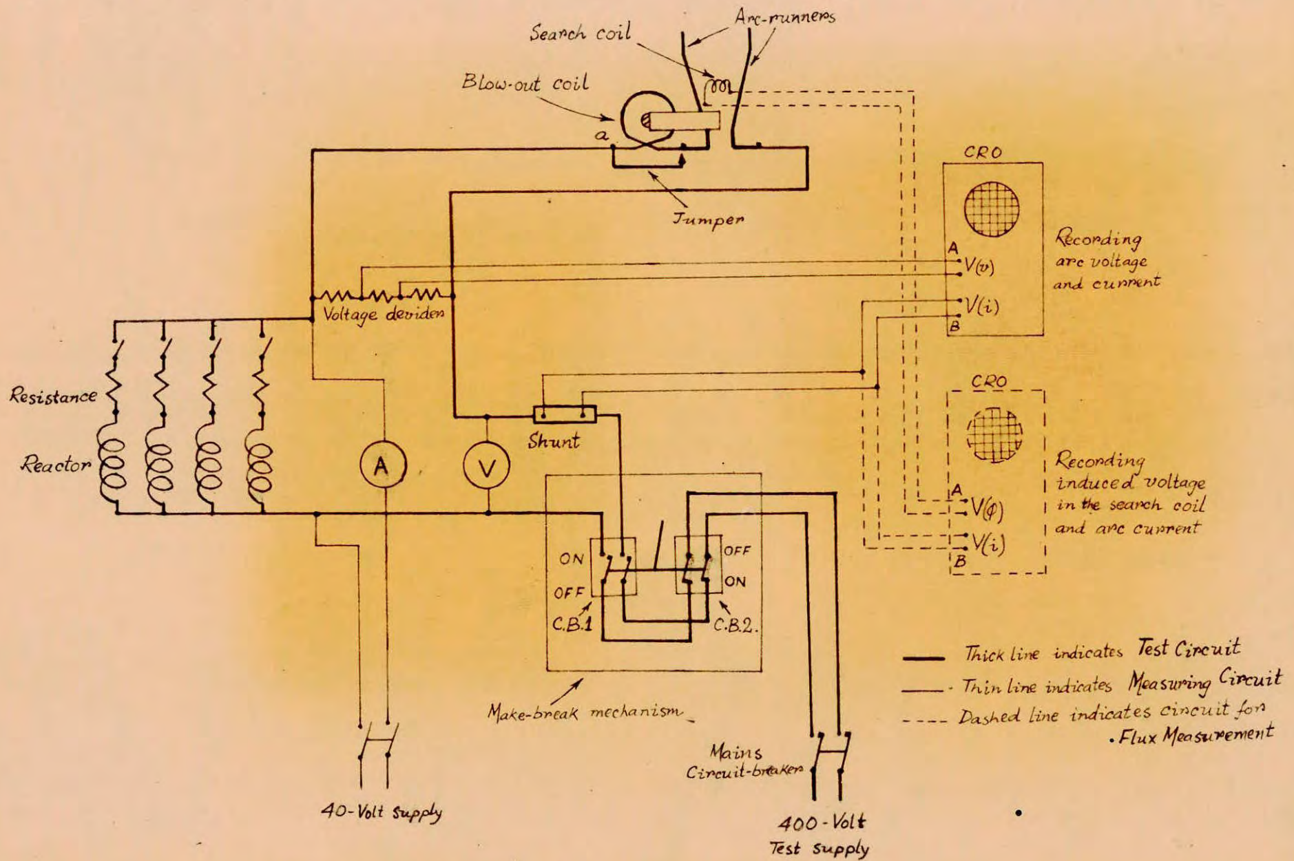
FIG. 20 Schematic diagram showing experimental set-up.
