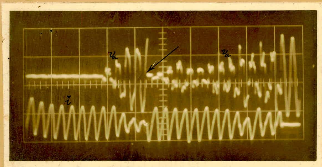
Fig 35(b) Oscillogram of a ' restriking'
