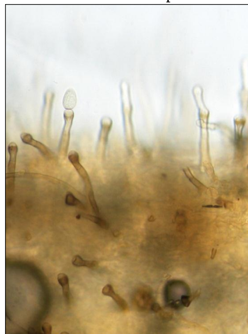
(e) Conidiophore
