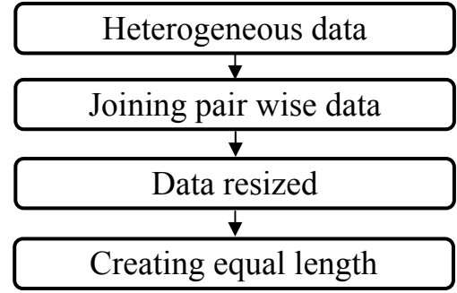
Figure 1: Data preprocessing
