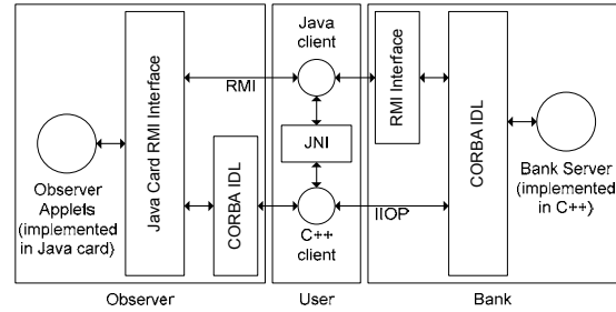
Fig. 5. Wallet with Java card observer and bank server component architecture.
