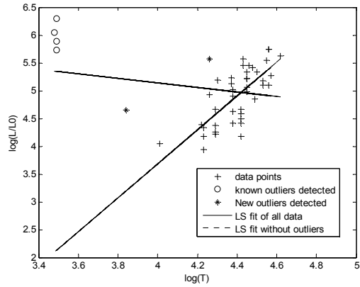
Fig. 4. The dataset, outliers, and least-squares fits with and without outliers for CYG dataset.
