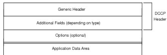
Fig. 3. DCCP packet structure
