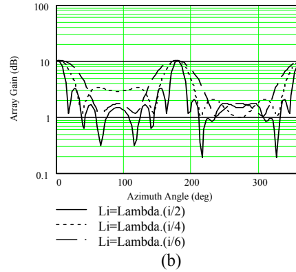
Fig. 6. The variation of antenna gain on Azimuth plane in polar and rectangular coordinate (seven adaptive element beam former).
