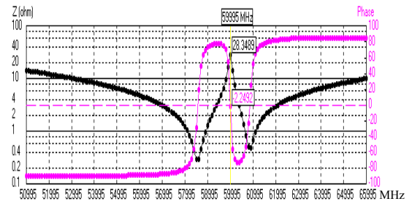
Fig 9. Impedance and phase of the antenna.
