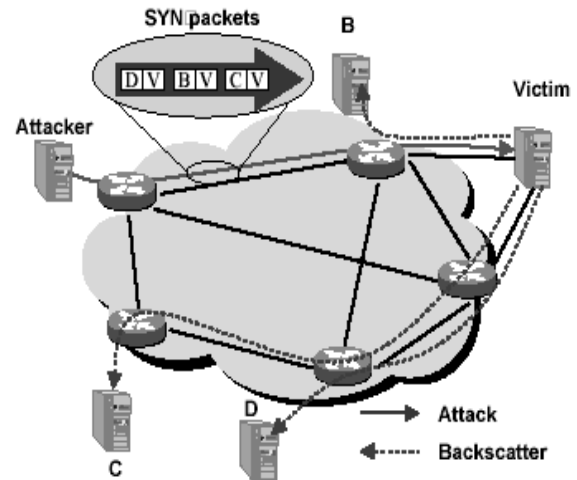
Figure 2: Backscatter
