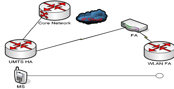
Fig. 1. Mobile IP showing session continuity with hand-over
