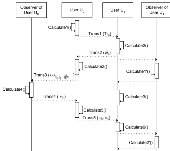
Fig. 4. User U_0 spends his coin to user U_1 .
