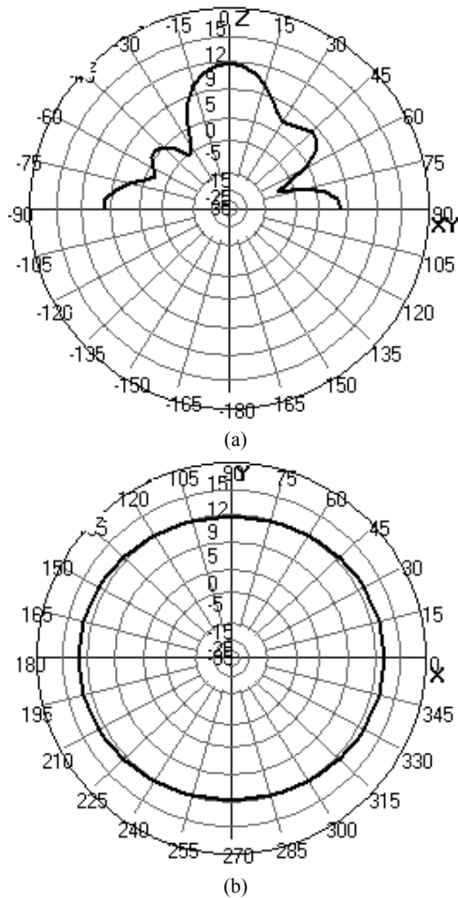
Fig. 13. Total gain pattern of stair ILA at 5.5 GHz in (a) vertical plane and (b) horizontal plane.
