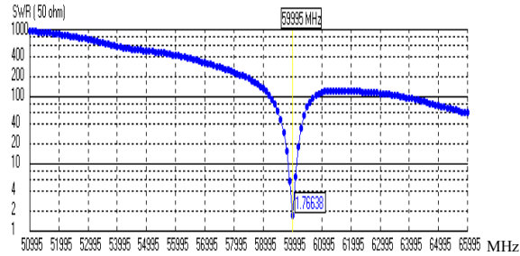
Fig. 4. Standing Wave Ratio (SWR) of the antenna.
