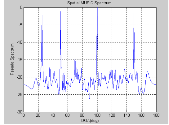
Fig. 9. Pseudo Spectrum of MUSIC with angle, Signal arrival at 25° and 50°, 100°, 150° and SNR is 18dB.
