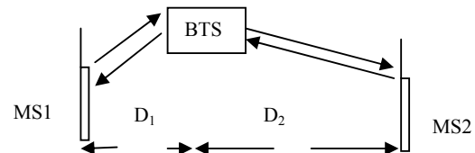
Fig3. Near-Far Effect
