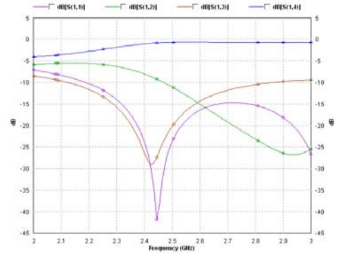
Fig. 4.S-parameters versus frequency at port 1.
