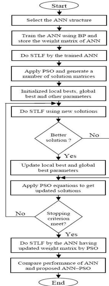
Fig. 4. Flowchart of the Proposed Algorithm
