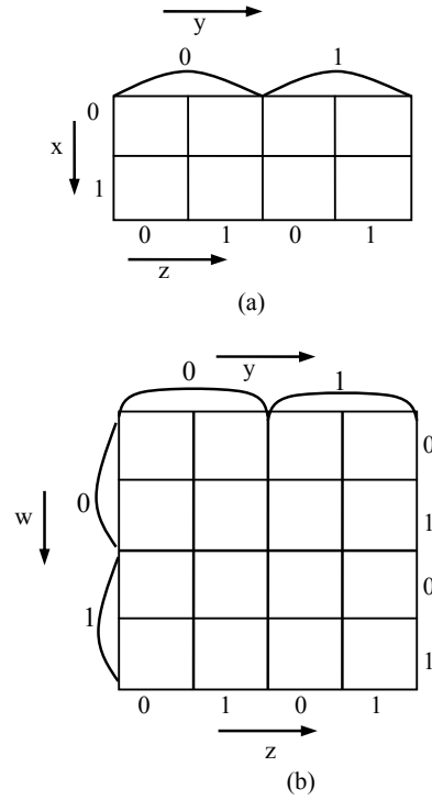
Figure 5: Realization of Boolean function using K-map
