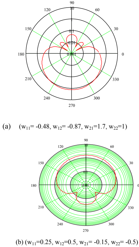
Fig. 4. Radiation Pattern of two reference antenna system.
