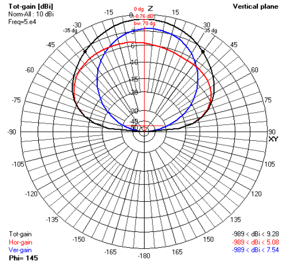
Fig. 2. Radiation pattern of the antenna.
