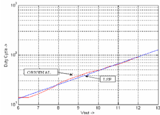
Fig. 12. Least Square Fit graph for V_{out} vs Duty Cycle
