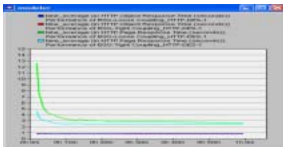
Fig. 9. HTTP response time
