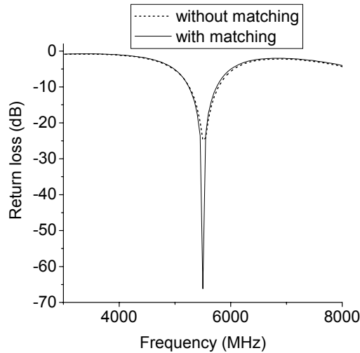
Fig. 5. Return loss of inverted-L antenna with frequency.
