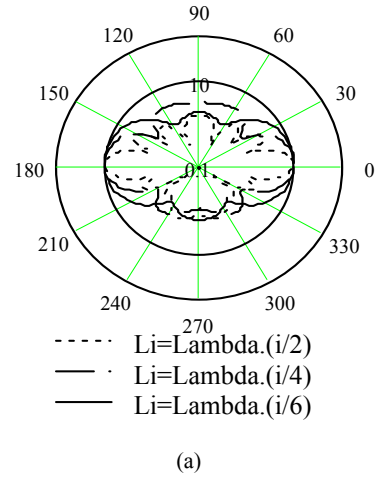
Fig. 5. The variation of antenna gain on Azimuth plane in polar and rectangular coordinate (two adaptive element beam former).
