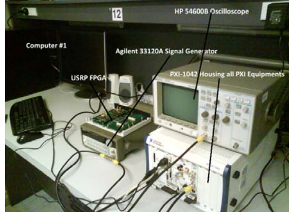
Fig. 3. Cognitive radio work bench
