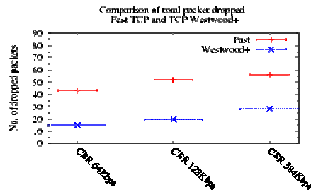
Fig. 3. Comparison of total no. of packet drops between Fast TCP and TCP Westwood+ at different CBR flows
