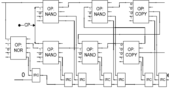
Fig. 7. Online testability of reversible D FF
