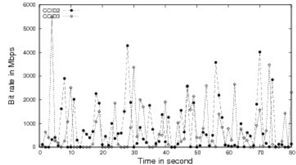
Fig. 13. Time vs Bit rate of CCID 2 and CCID 3 on 10% loss
