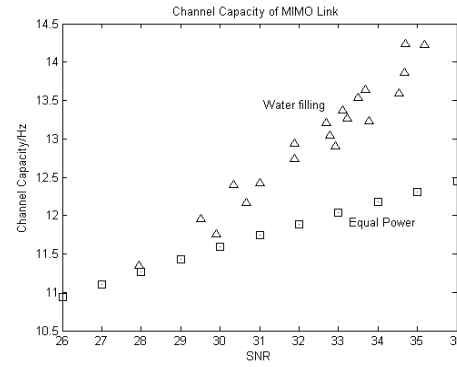
Fig. 3. Channel capacity versus SNR ( \mu=1.7 ).
