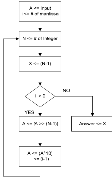
Fig. 1. Algorithm for the computation of decimal logarithm
