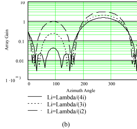
Fig. 5. The variation of antenna gain on Azimuth plane in polar and rectangular coordinate (two adaptive element beam former).
