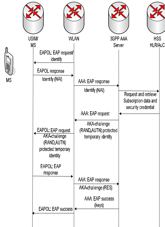
Fig. 2. EAP-AKA Procedure
