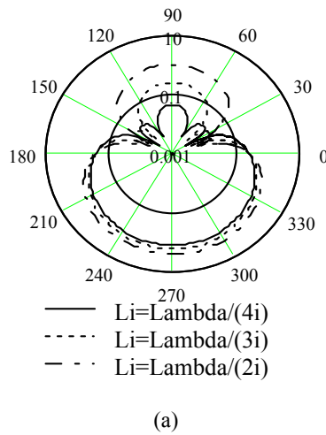
Fig. 4. Radiation Pattern of two reference antenna system.
