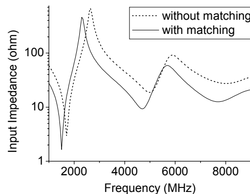
Fig. 8. Input impedance variation of inverted-L antenna.
