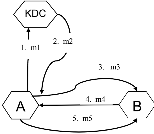
Fig.3. Conventional Needham-Schroeder Key Distribution Protocol
