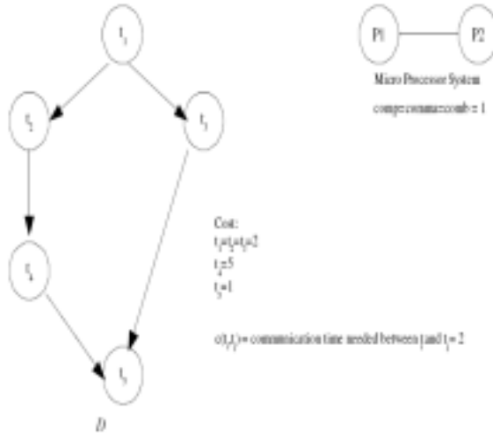
Fig 1: Task graph to be scheduled on processor P_1 and P_2
