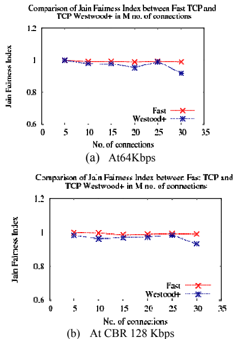
Fig 10. Comparison of Jain Fairness Index for some Fast TCP and TCP Westwood+ connections (a), (b)
