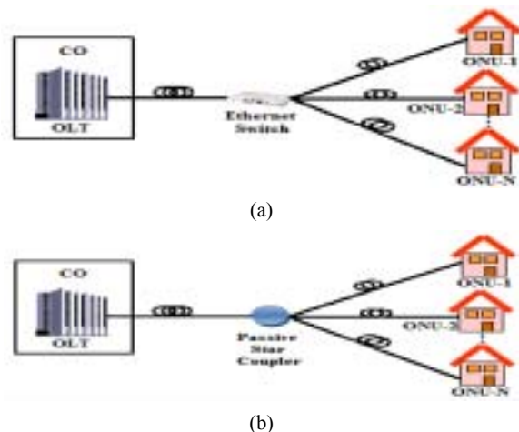
Fig. 2. Optical Networks. (a) Active Optical Network (AON); (b) Passive Optical Network (PON)
