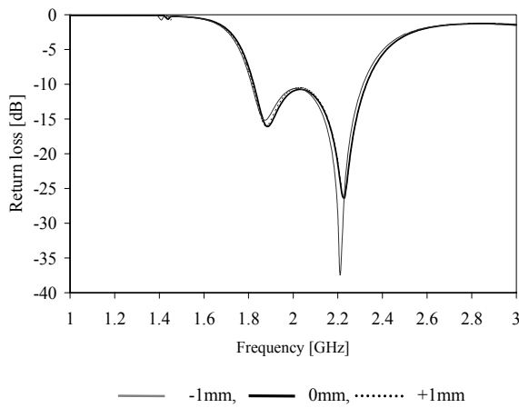
Fig. 5. Effect on return loss of different slot width ( w_l ) of the proposed patch.
