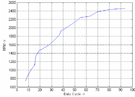
Fig. 7. Actual graph for Duty Cycle vs RPM (Forward Direction)
