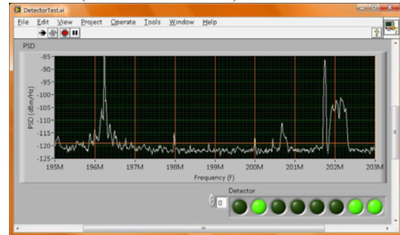
Fig. 1. Energy detector performance on narrow band signals
