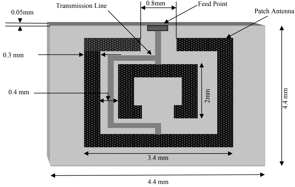
Fig. 1. Antenna configuration.
