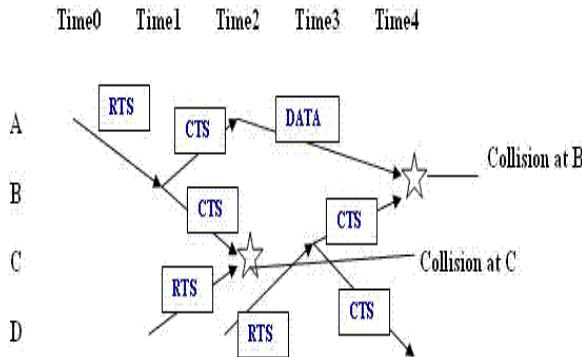
Figure-1: Hidden terminal problem after using RTS/CTS control packets
