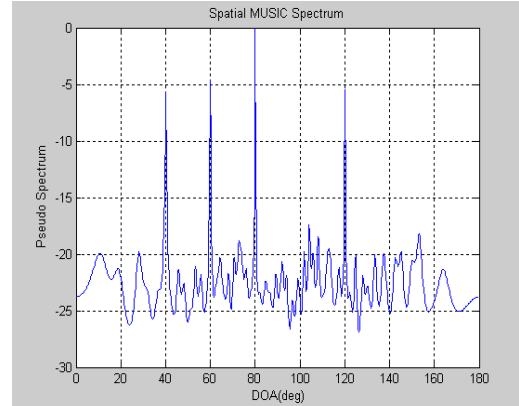
Fig.10. Pseudo Spectrum of MUSIC with angle, Signal arrival at 40°, 60°, 80° and 120° SNR is 16dB.
