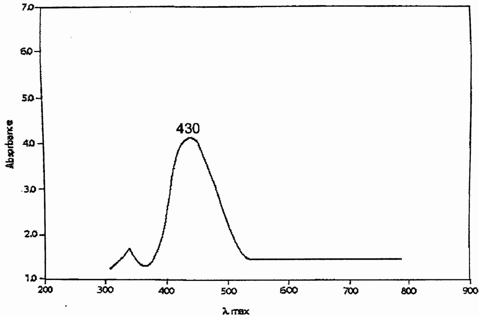
Fig.-7.1 : UV-Visible spectrum of K^+[V(IV) (Mal)_2 (\beta\text{-Ph-ala})]^- Complex-1
