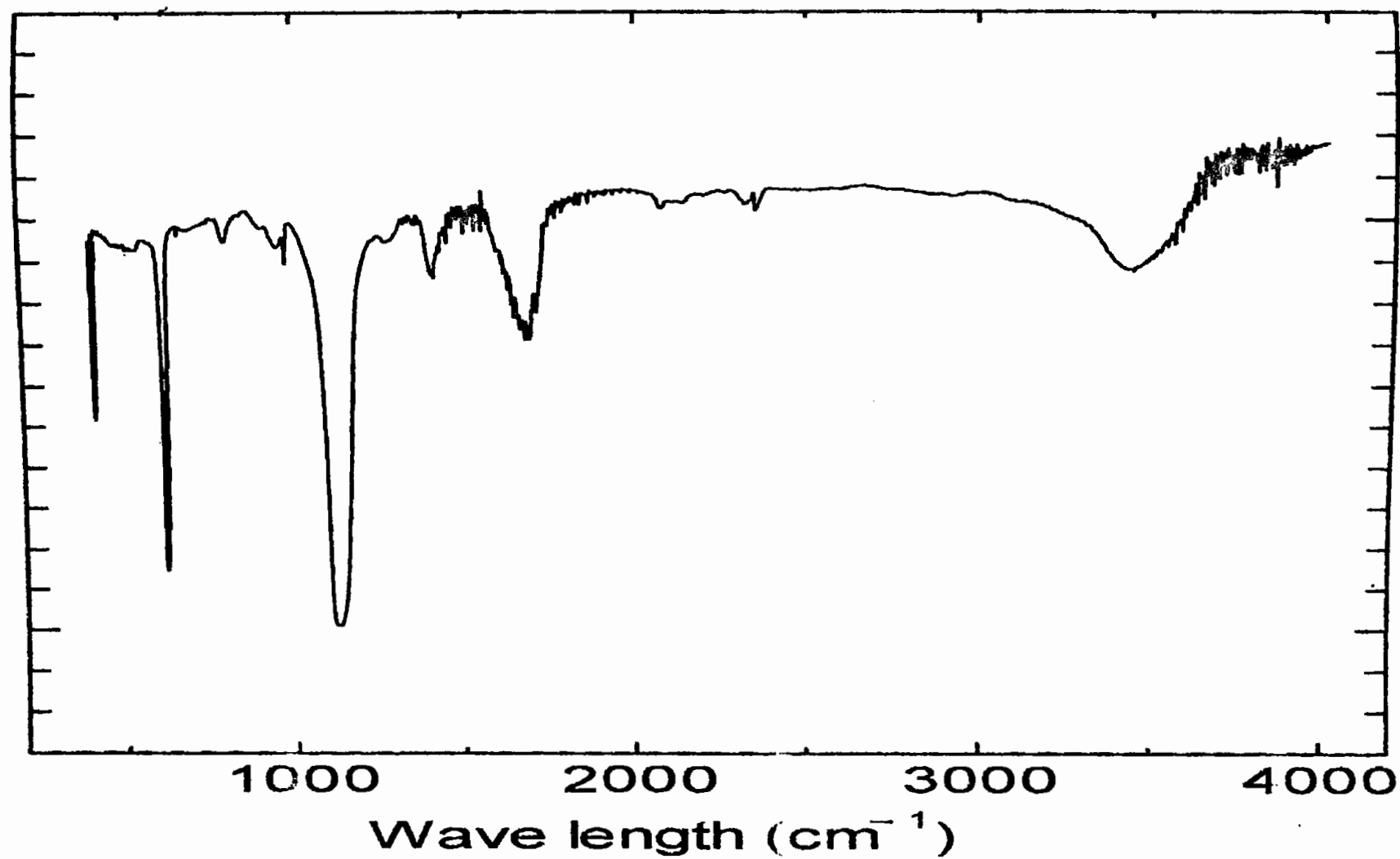
Fig. 6.1: IR spectrum of \text{K}^+[\text{V(IV)(oxa)}_2(\text{ala})]^-
