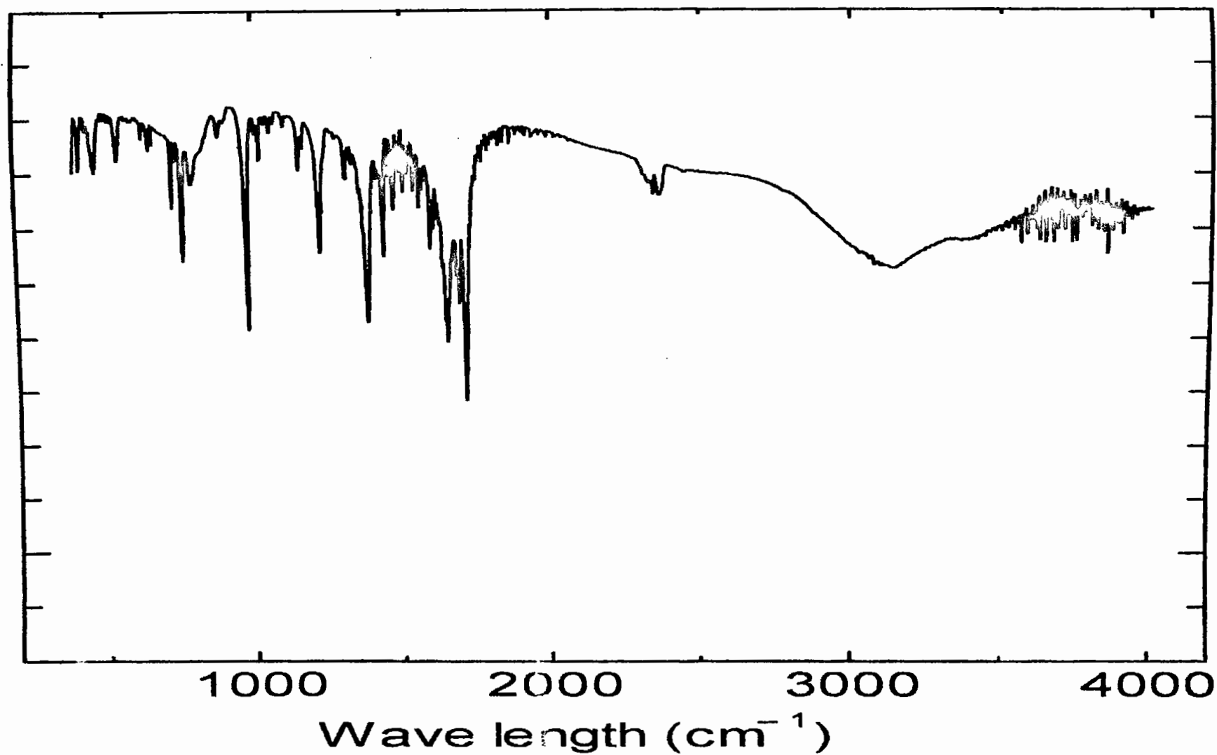
Fig. 6.3: IR spectrum of \text{K}^+[\text{V(IV)(oxa)}_2(2,2'\text{-Bipy})]^-
