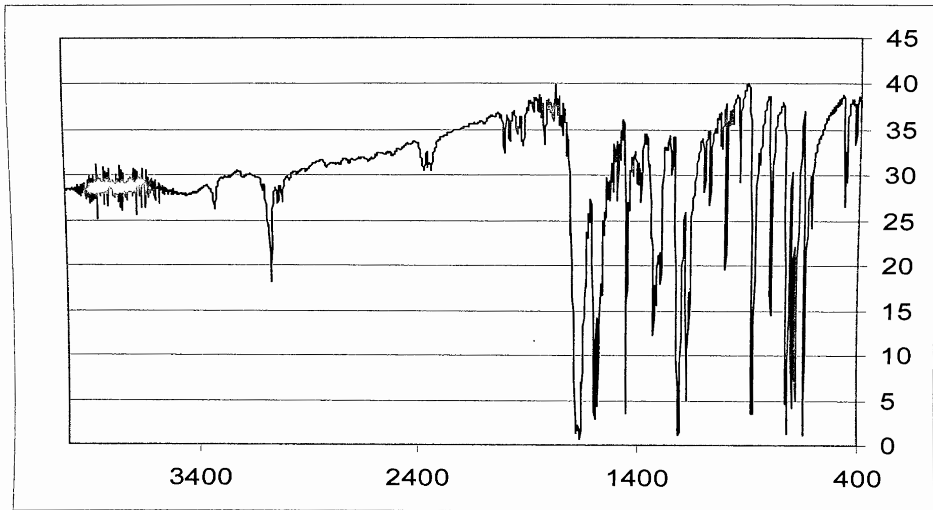
Fig. 5.3: IR spectrum of \text{K}[\text{Zr(IV)(Mal)}_2(\text{ala})]^-
