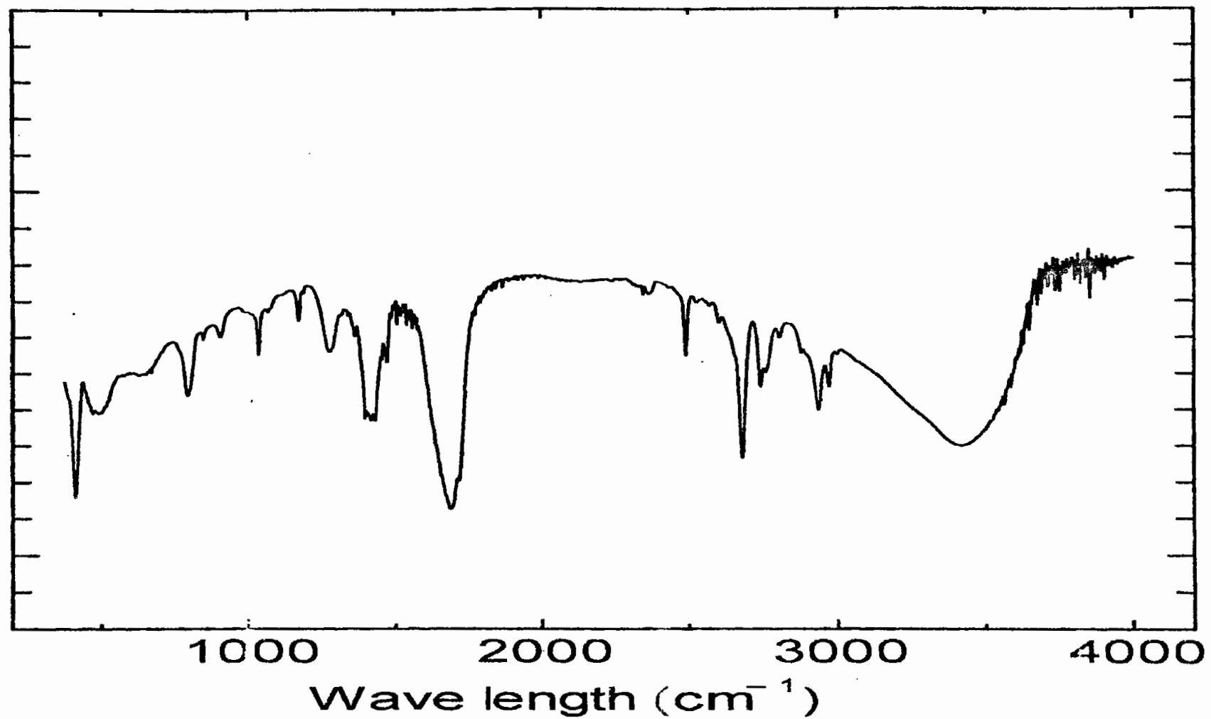
Fig. 3.4: IR spectrum of [Zr(IV)(oxa) 2 (Py) 2 ]
