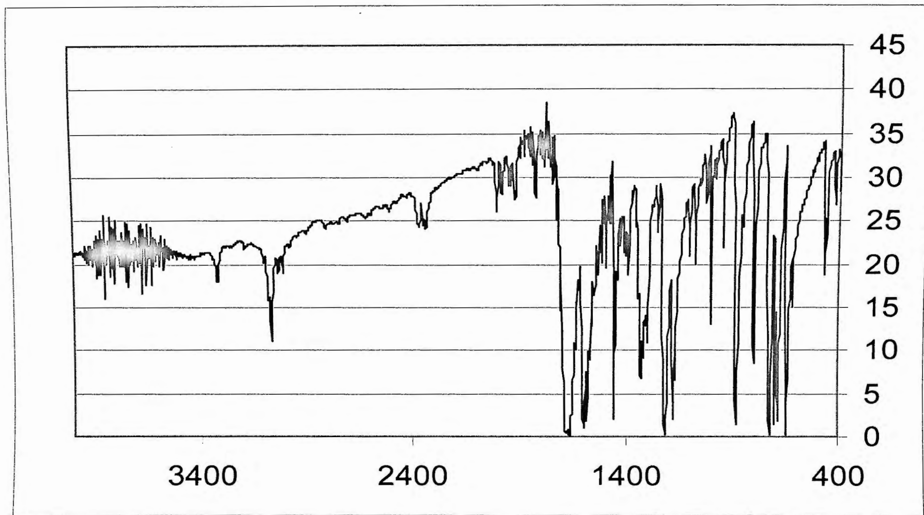
Fig. 5.4: IR spectrum of \text{K}[\text{Zr(IV)(Mal)}_2(\beta\text{-ph-ala})]^-
