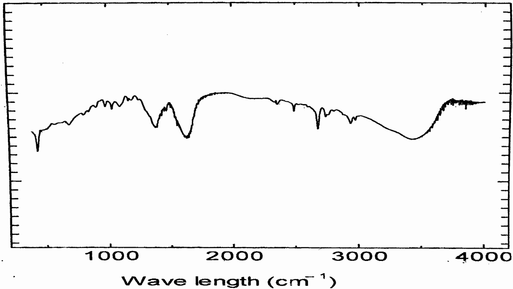
Fig. 4.3: IR spectrum of [Zr(IV)(Mal) 2 ( \alpha -Pic) 2 ]
