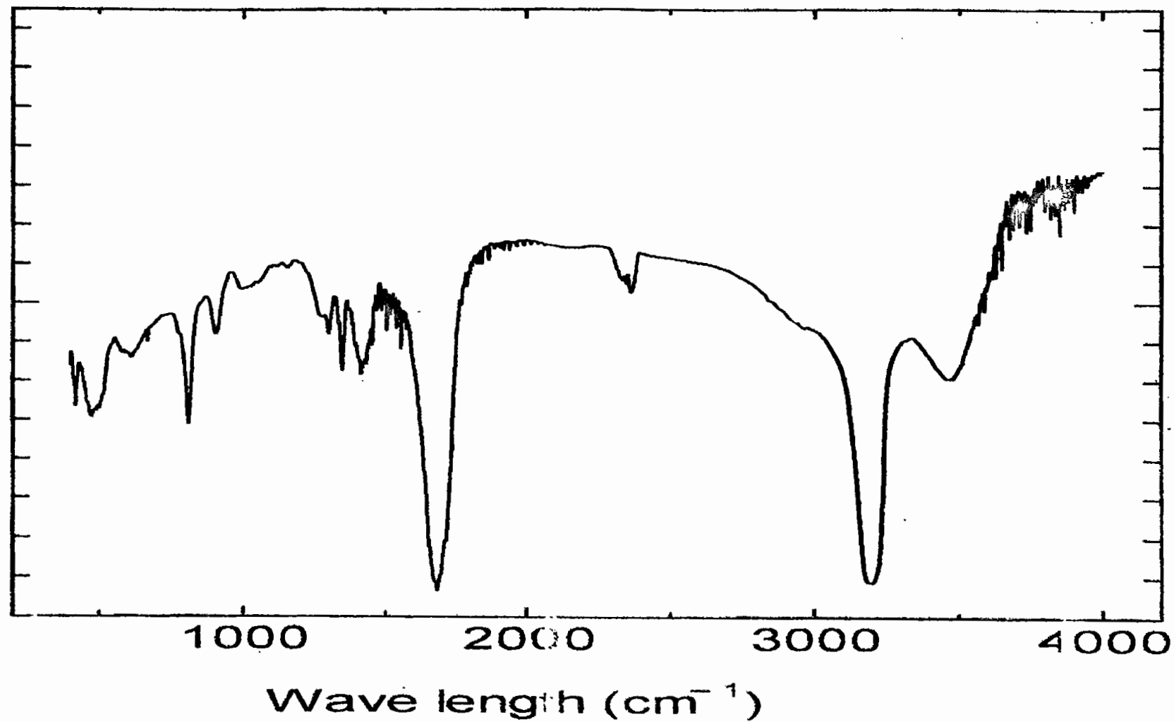
Fig. 3.1: IR spectrum of [\text{Zr(IV)(oxa)}_2\text{Q}_2]
