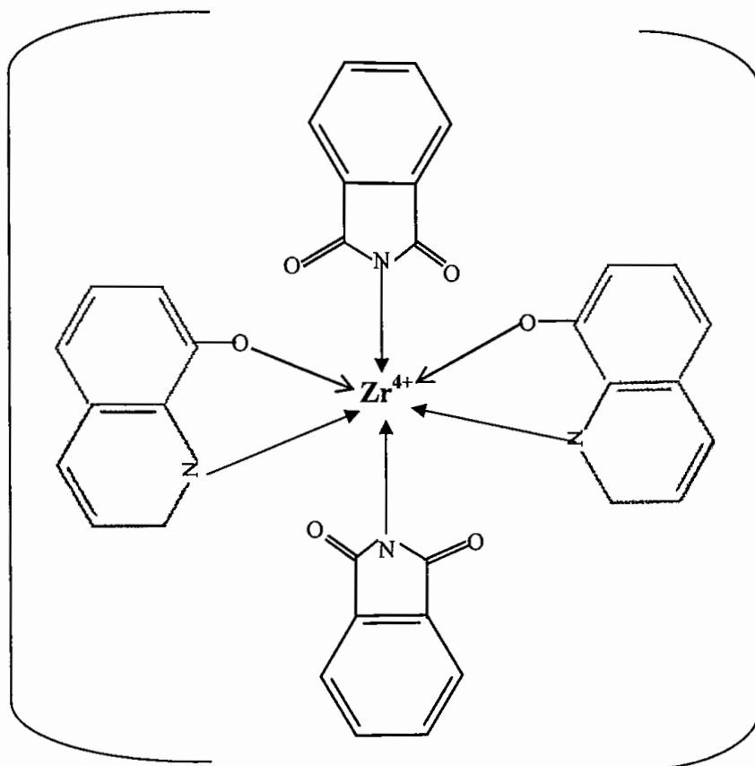
Fig 8.1: Possible structure of the complex [Zr(IV) (Phtha)_2 (8-HQ)_2]
