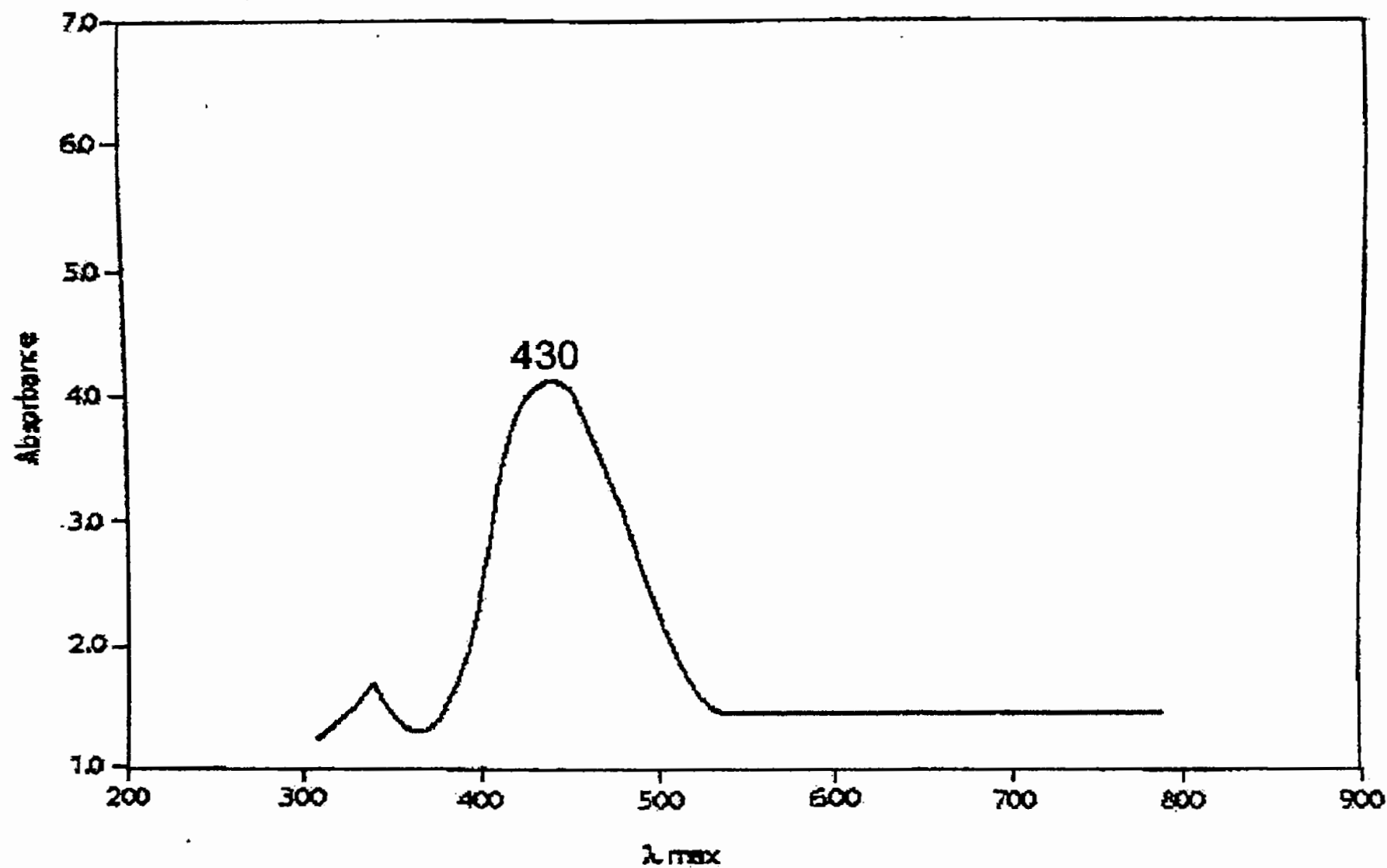
Fig.-6.4 : UV-Visible spectrum of K^+[V(IV) (oxa)_2 (ala)]^- Complex-1
