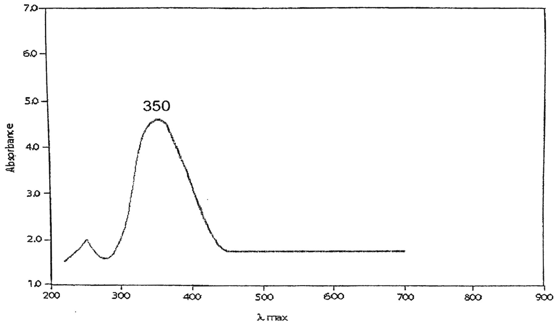
Fig.-4.4: UV-Visible spectrum of 2K^+[Zr(IV) (Mal)_2 (8-HQ)_2]^{2-} Complex-1
