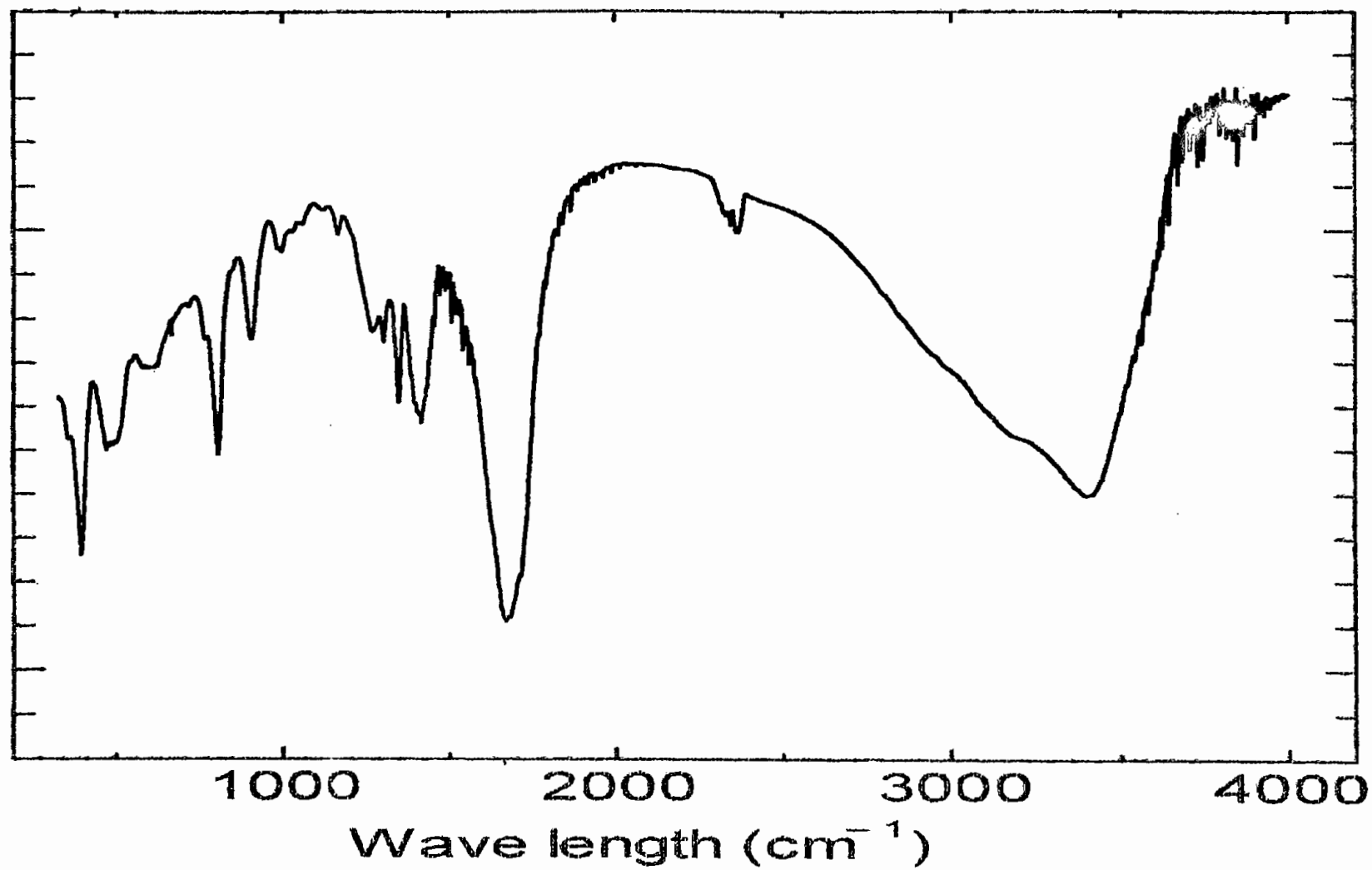
Fig. 3.2: IR spectrum of [\text{Zr(IV)(oxa)}_2(2\text{-Apy})_2]
