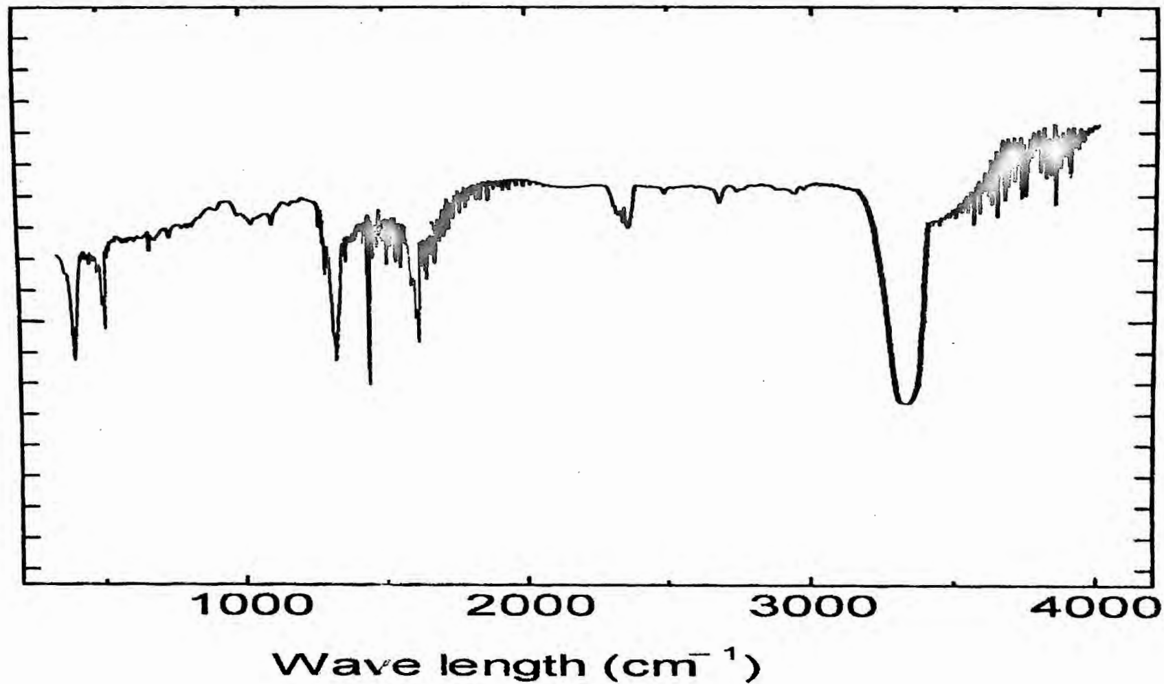
Fig. 4.1: IR spectrum of 2k^+[\text{Zr(IV)}(\text{Mal})_2(8\text{-HQ})_2]^{2-}
