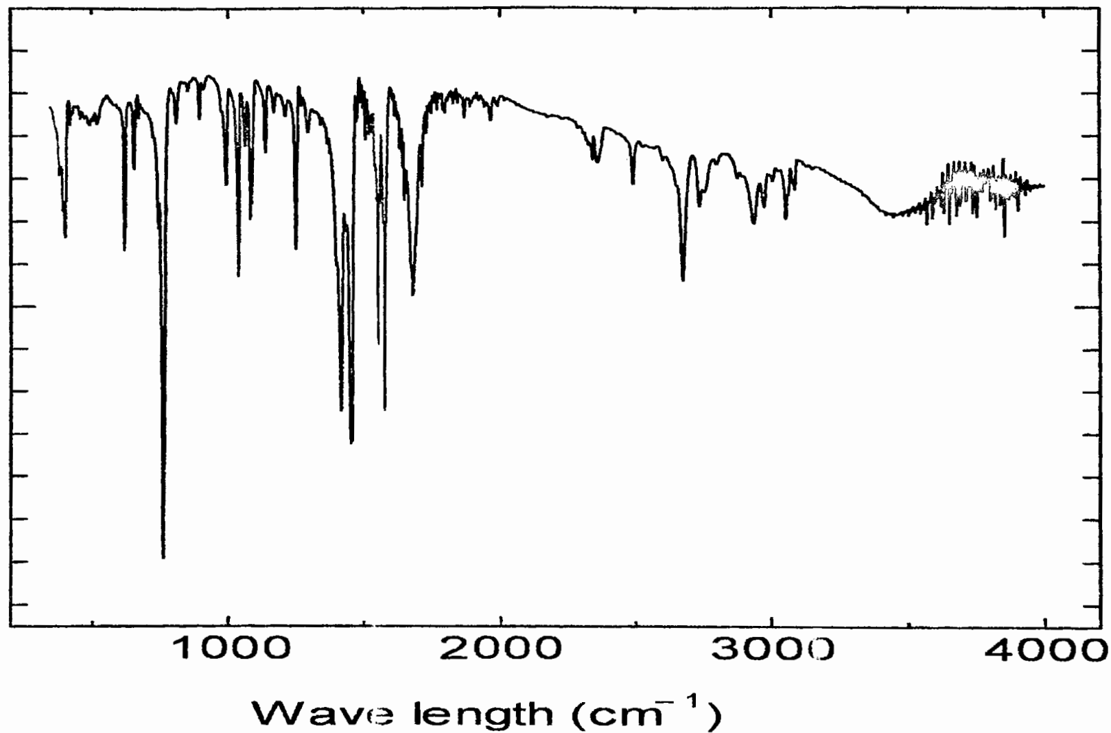
Fig. 3.5: IR spectrum of [\text{Zr(IV)(oxa)}_2(2,2'\text{-Bipy})_2]
