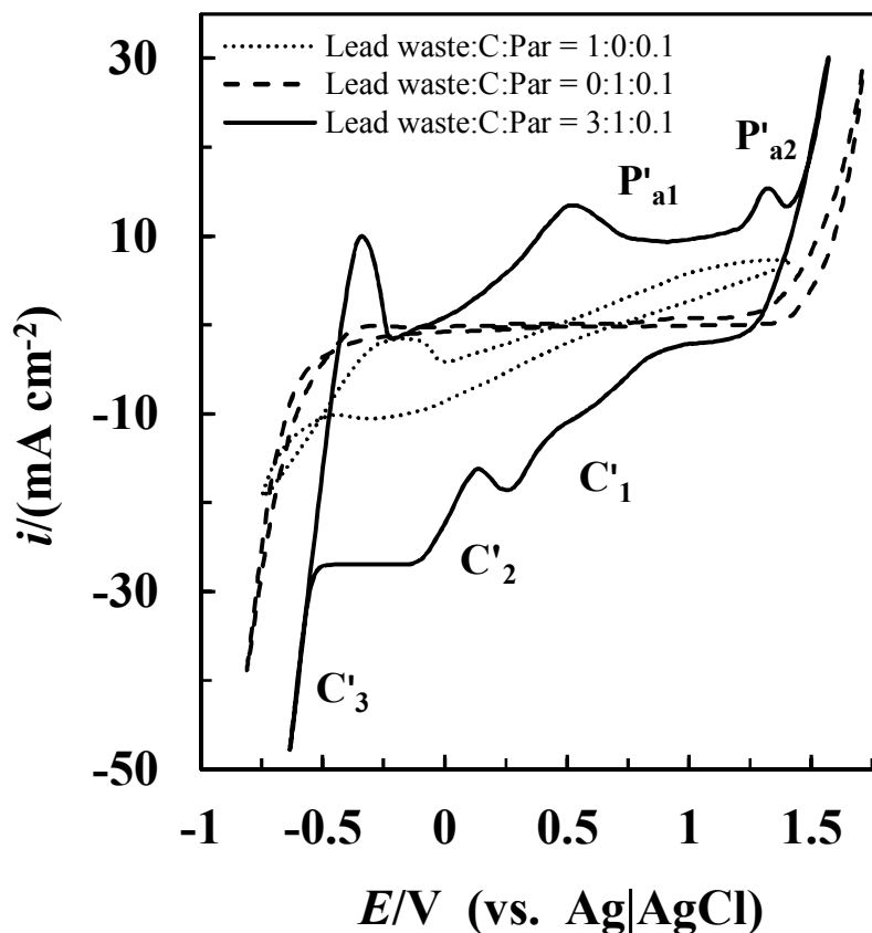
Figure 5.27 Cyclic voltammograms recorded on a pellet of waste lead, graphite and paraffin mixed electrode in 1 mol dm -3 HNO 3 at 30° C with a scan rate of 10 mV s -1 .
