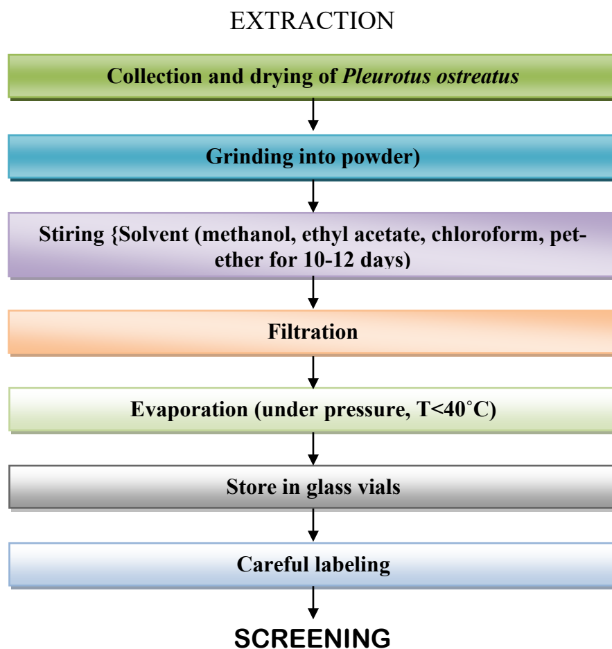
Figure-3.1: Pathway of extraction (organic solvents).
