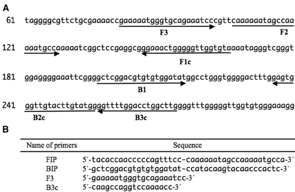
Fig. 3.1 Primers and their locations for amplification of Leishmania donovani kinetoplast minicircle DNA by LAMP. A - locations of the primer sequences. B - names and sequences of four primers. Primer FIP consists of F1 complementary sequence and F2 direct sequence. Primer BIP consists of B1 direct sequence and B2 complementary sequence.
