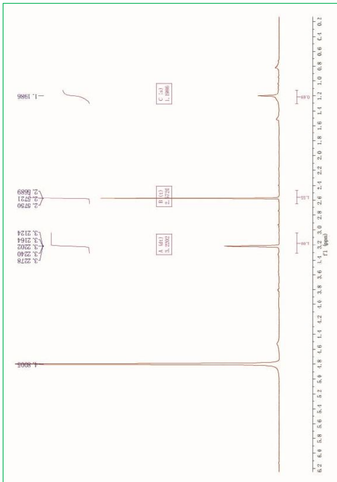
Fig. 3.2: ^1\text{H} NMR spectrum of Po. hydropiper (wp) compound 2 (POM)
