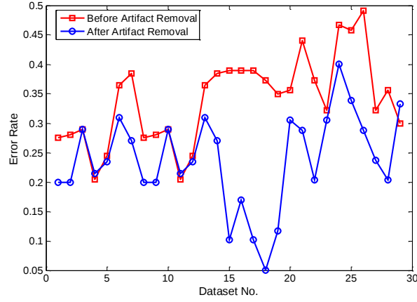
Figure 6.13: Error Rate for signals before and after artifact removal from the BCI output using LDA Classifier and Windowed Means as features from BCILAB tool.
