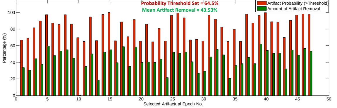
Figure 6.8: Selected epochs with probability more than threshold for artifact correction and their corresponding amount of artifact removal in %.
