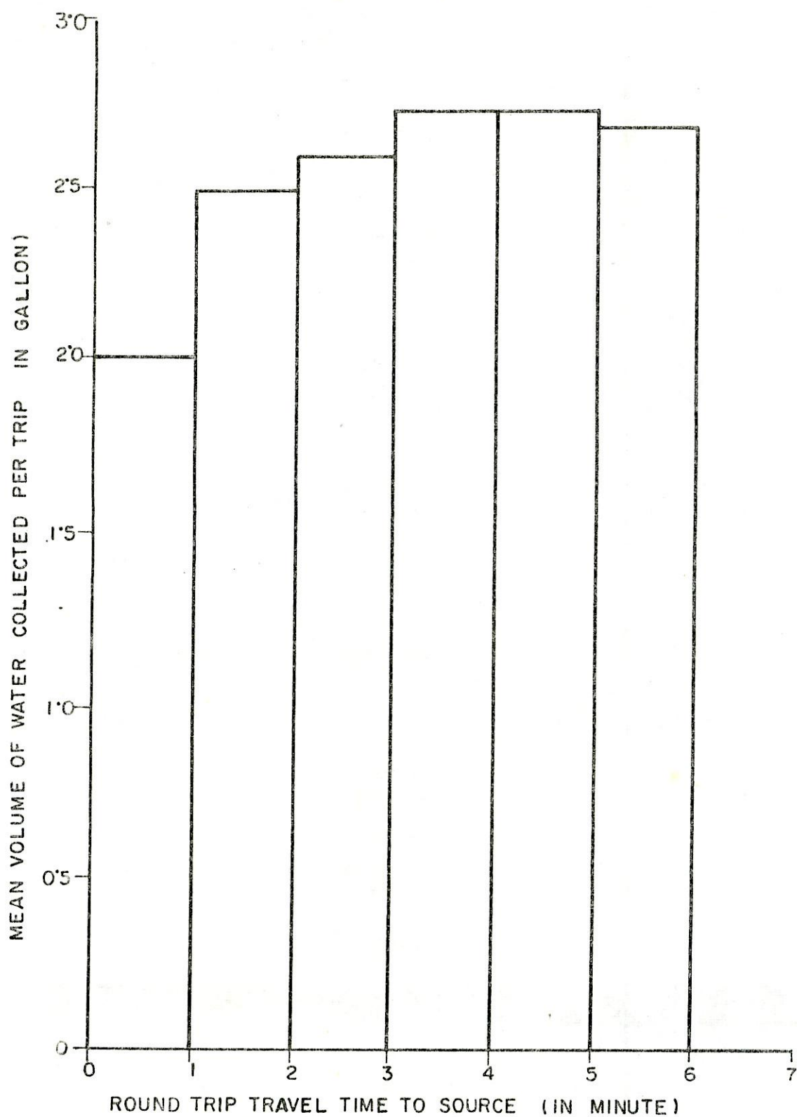
Fig. 4.5(a) Effect of Travel Time to Source on Volume of Water Collected Per Journey from Tubewell with No.6 Pump
