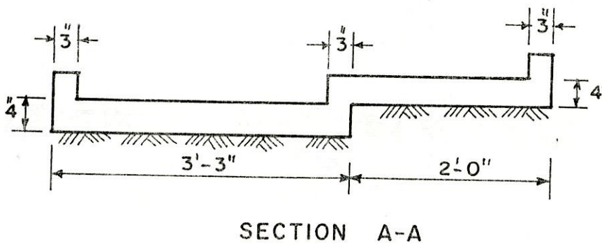
Fig. 4.15 Showing the Detail Drawing of Existing and Extended Platform.
