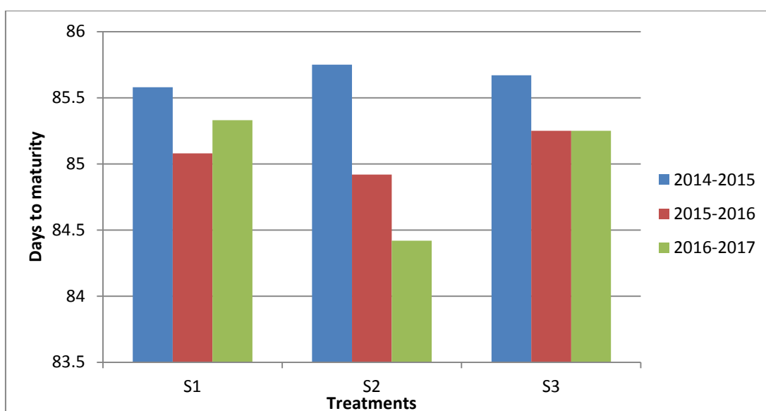
Figure 37. Effect of sowing time on days to maturity of mustard in the growing seasons of 2014-2015, 2015-2016 and 2016-2017 in farmer's field.
