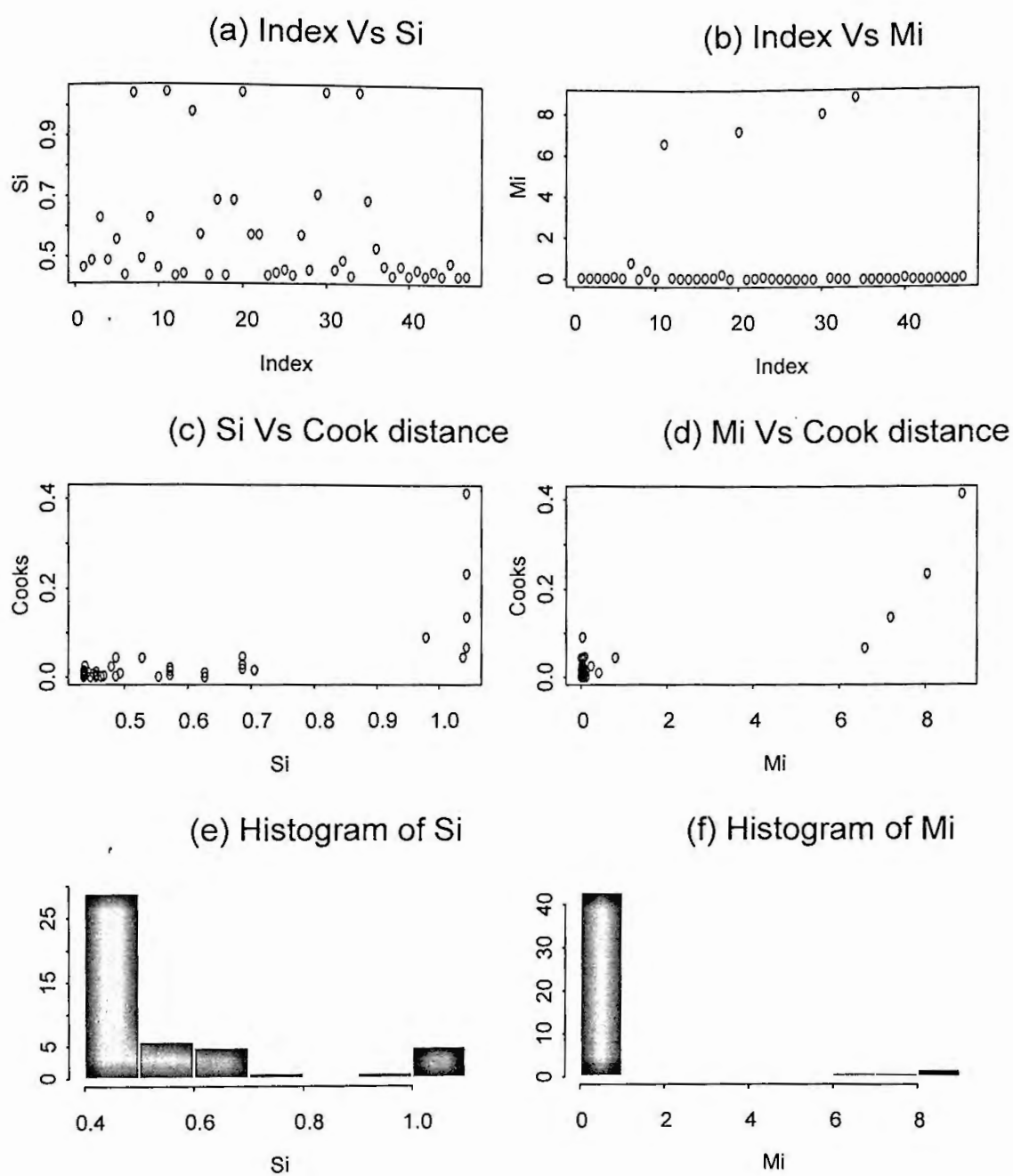
Figure 4.10 Index plots and Histograms of Influence measures for Hurtgsprung-Rusel Diagram data
