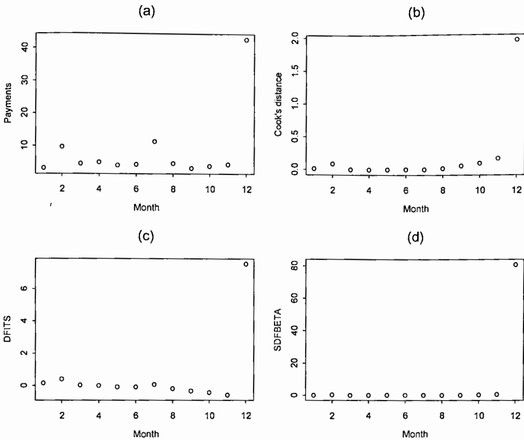
Figure 4.1 (a) Scatter plot Months versus Employment Payments; (b) Index plot of Cook's distance; (c) Index plot of DFFITS; (d) Index plot of SDFBETA
