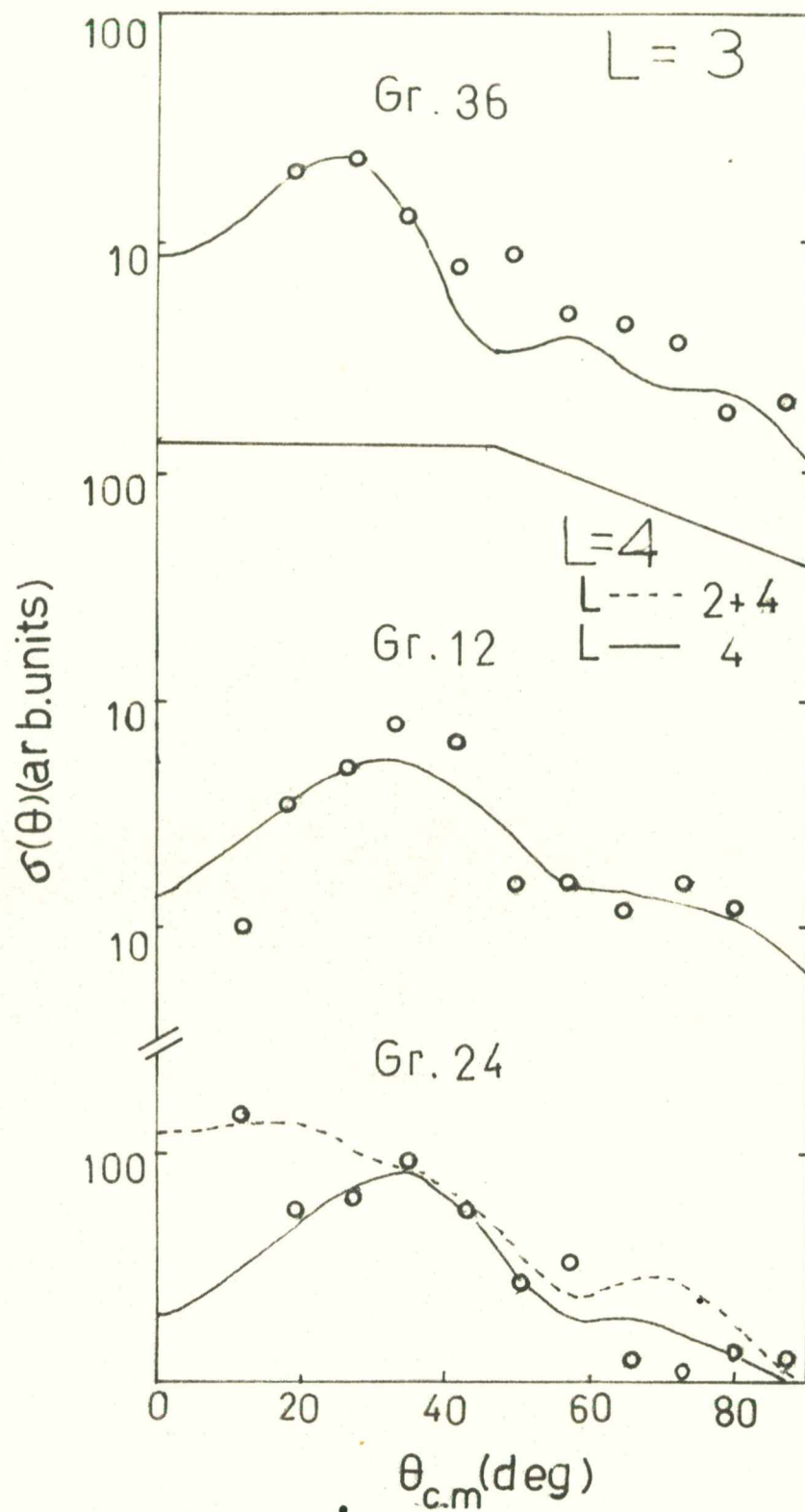
FIG. 6.5. Experimental angular distributions fitted to L = 3 and 4 DWBA curves.
