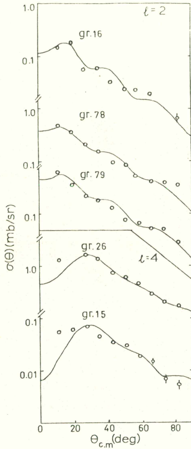
FIG. 4.5. Measured angular distributions fitted with \ell=2 and 4 DWBA curves.
