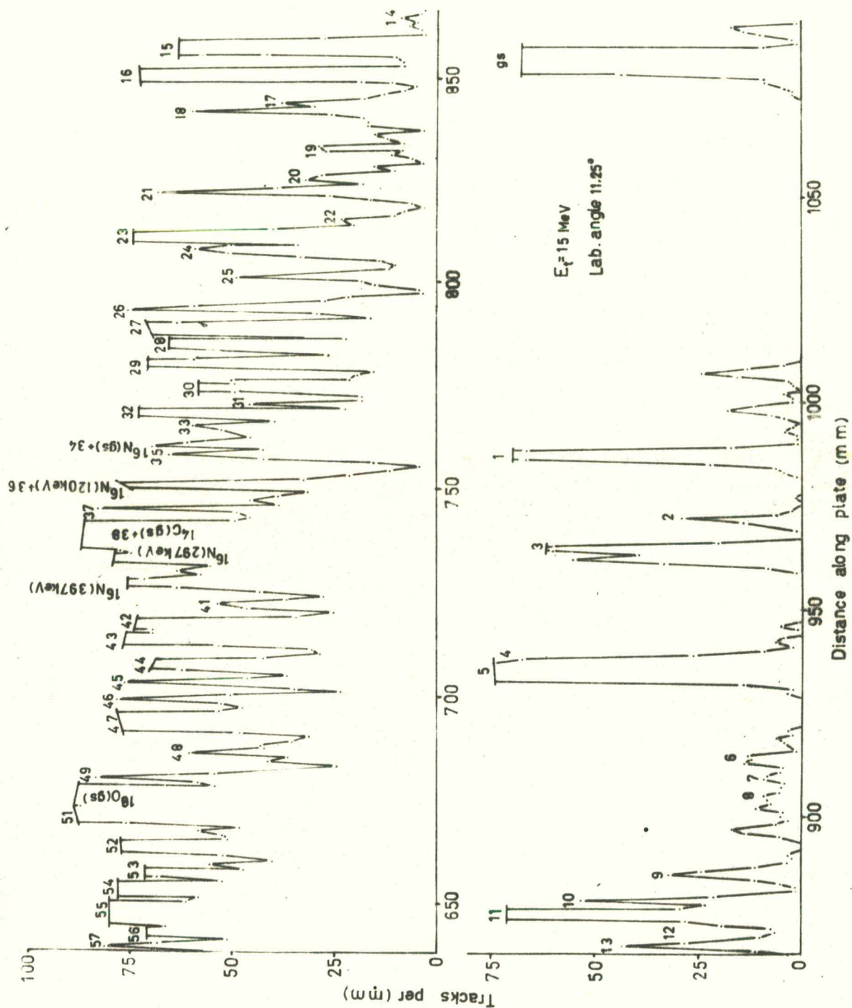
FIG. 6.1. Proton spectrum from ^{59}\text{Co}(t,p) reaction at 11.75^\circ .
