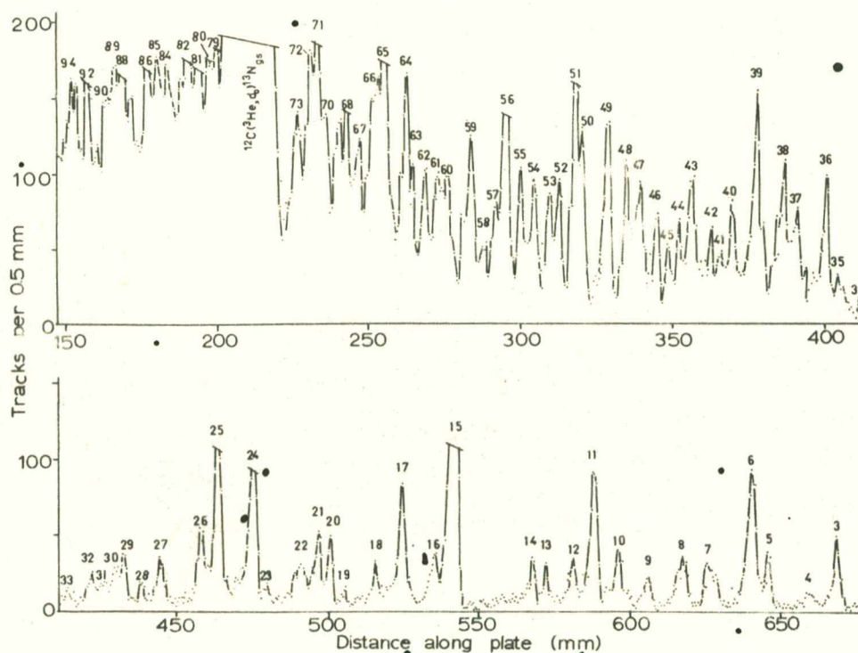
Fig. 1. Part of the energy spectrum of deuterons arising from the ^{45}\text{Sc}(t, d) reaction at 26.25^\circ showing the region of high density.
