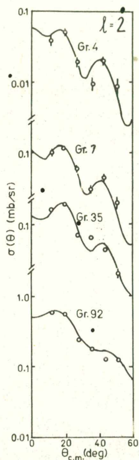
Fig. 6. Measured angular distribution fitted with l = 2 DWBA curves.
