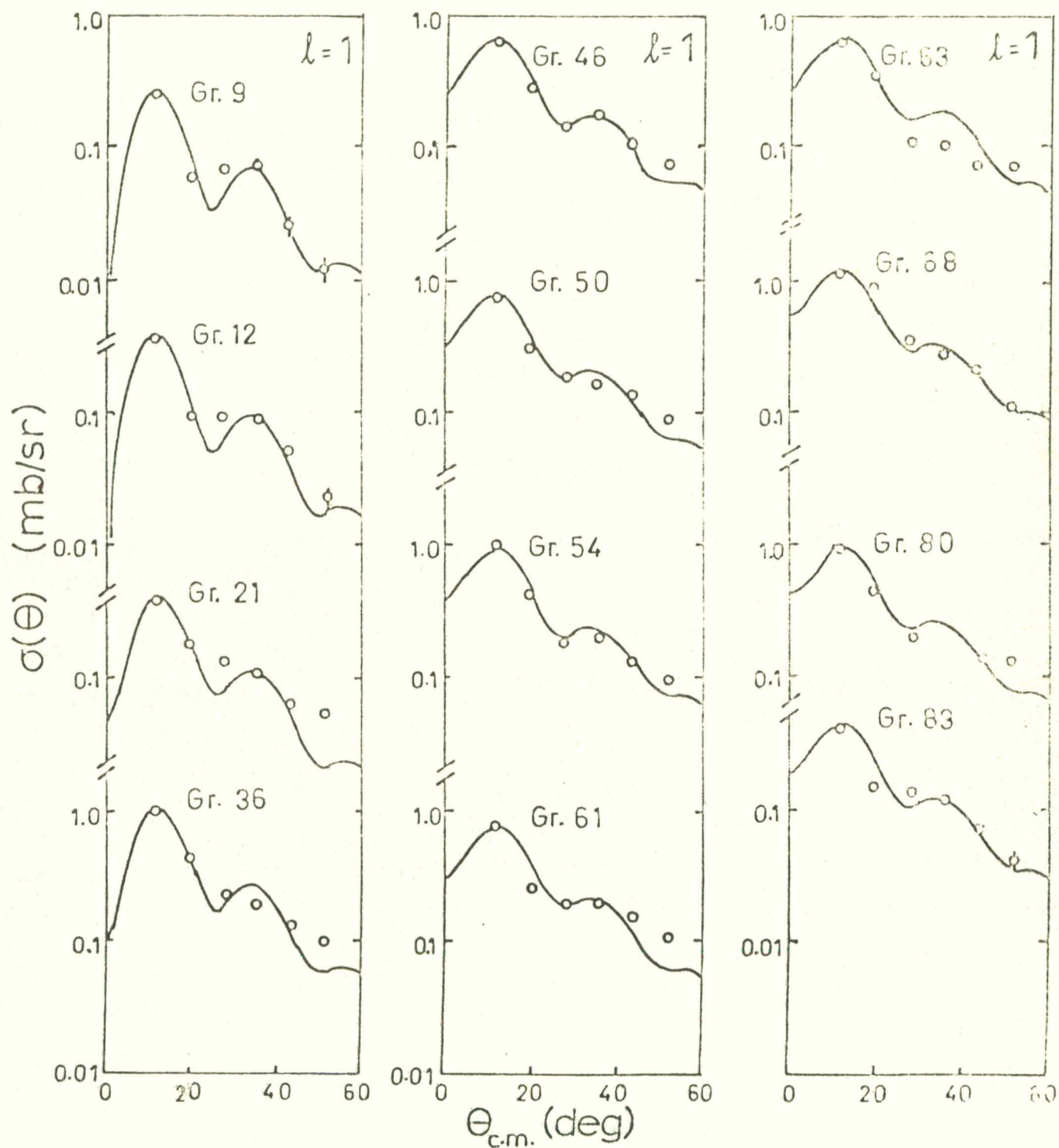
FIG. 5.2. Measured angular distributions fitted with l = 1 DWBA curves.
