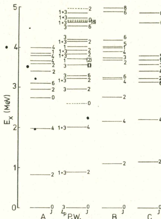
Fig. 8. Experimental level spectrum of ^{46}\text{Ti} compared with theory (only positive-parity levels shown). P.W.: Present work [levels with I_p = 3 character are shown by solid lines and other positive-parity levels are shown by broken lines; the J -values are from refs. 9-11 ]. (A) ref. 18 ), (B) ref. 5 ), (C) ref. 16 ).
