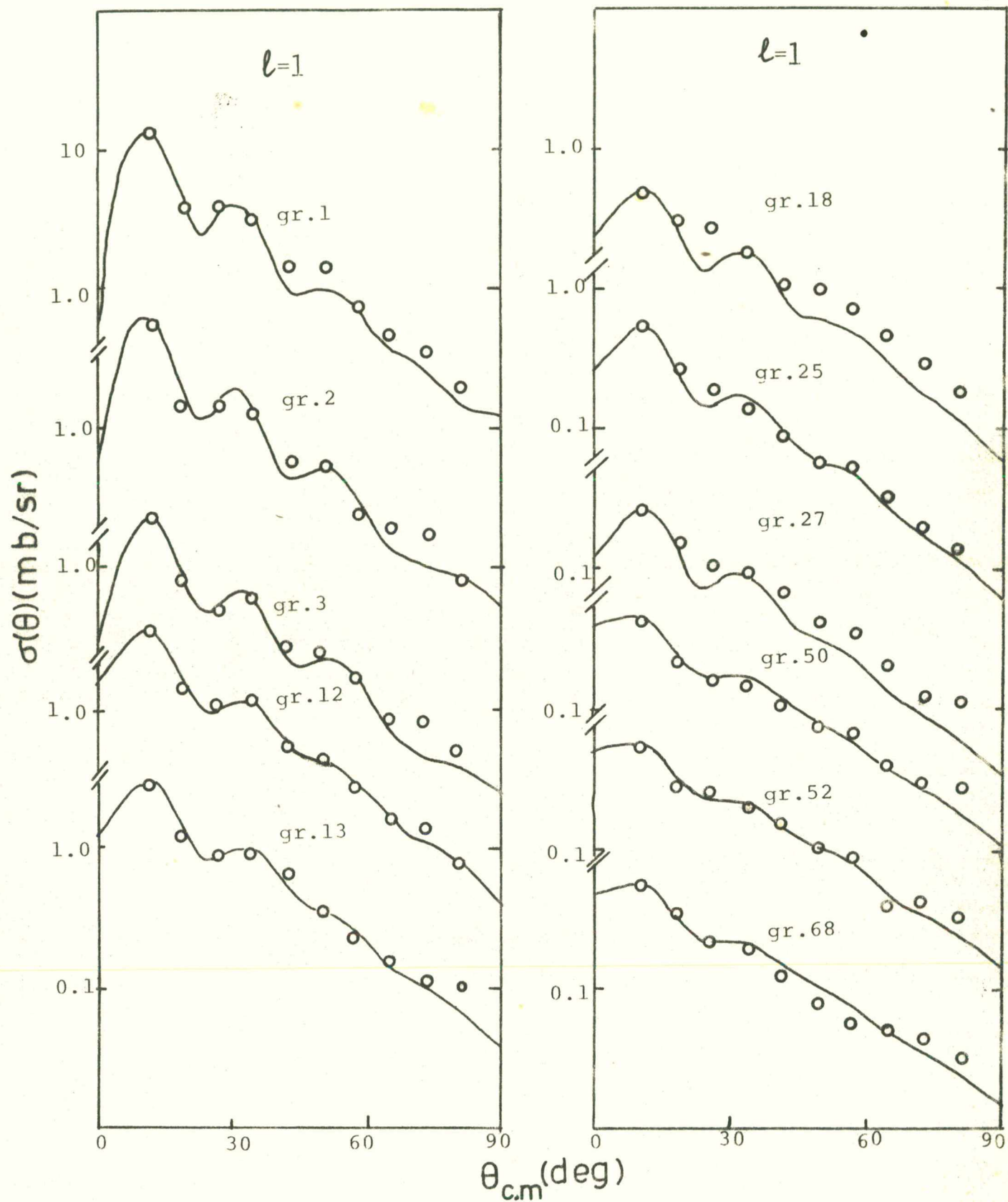
FIG. 4.2. Measured angular distributions fitted with l=1 DWBA curves.
