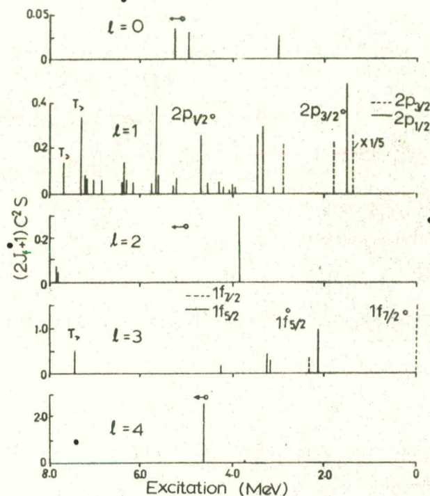
Fig. 5. The spectral distributions of single-particle strengths: the centre of the different T_c states are also shown.
