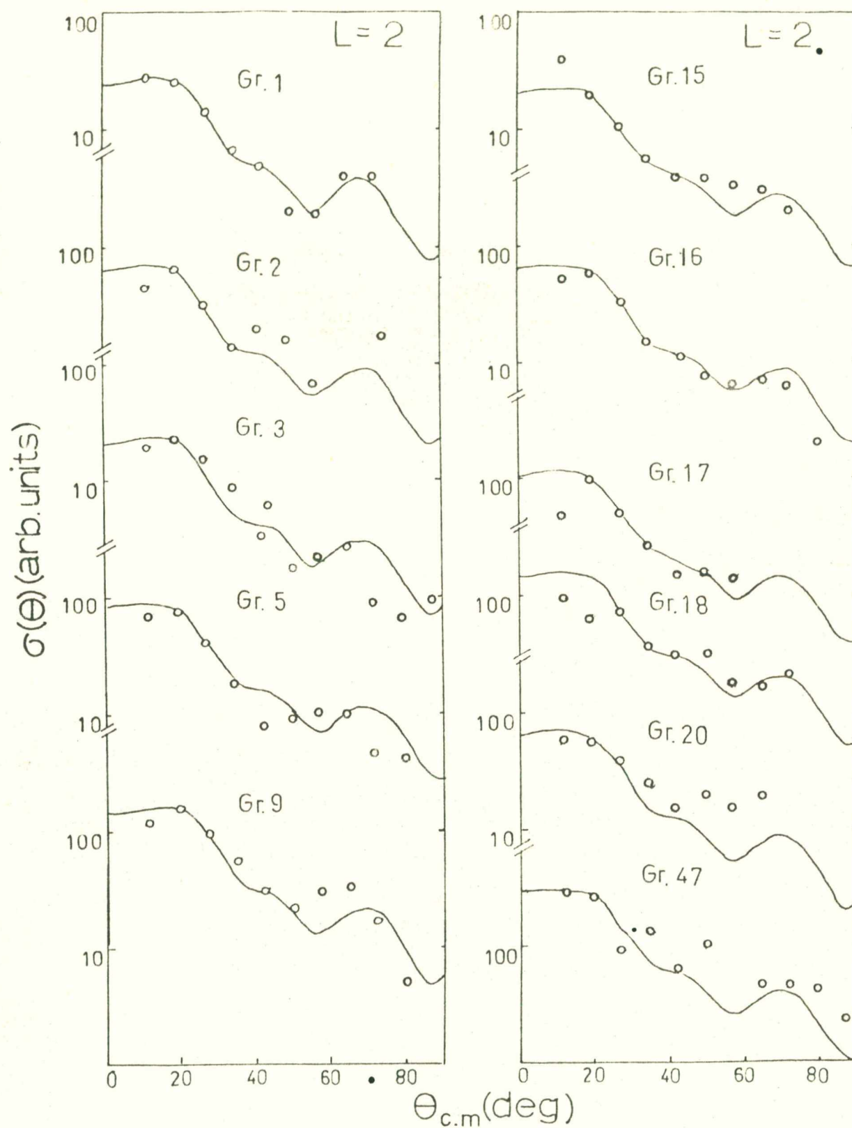
FIG. 6.4. Experimental angular distributions fitted with L=2 DWBA curves.
