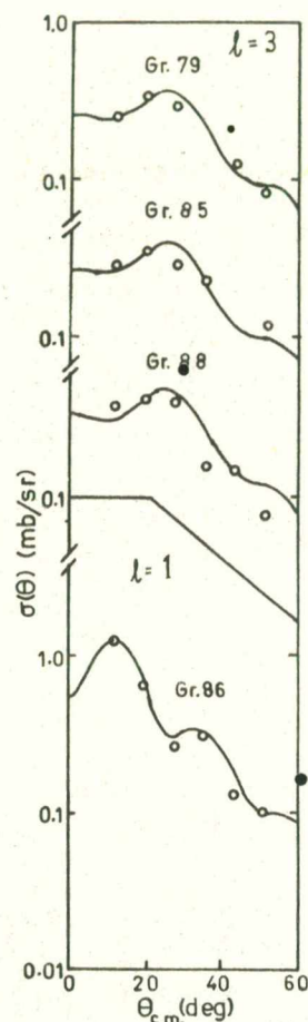
Fig. 7. Measured angular distribution for analogue states.
