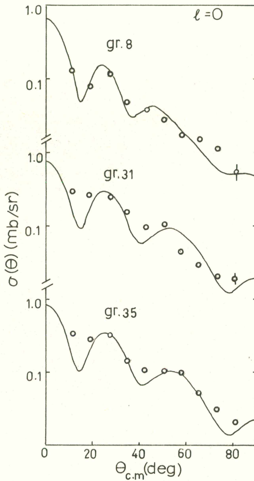
FIG. 4.4. Measured angular distributions fitted with l = 0 DWBA curves.
