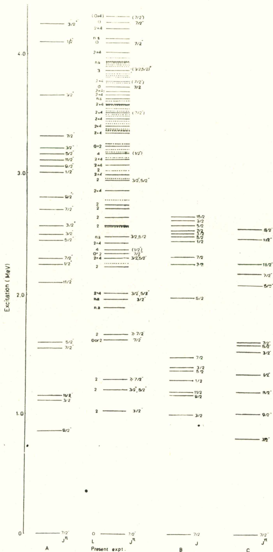
FIG. 6.10. Experimental level spectrum of ^{61}\text{Co} compared with theoretical calculations. A: (Sa 68). B: (St 71). C: (Go 72).
