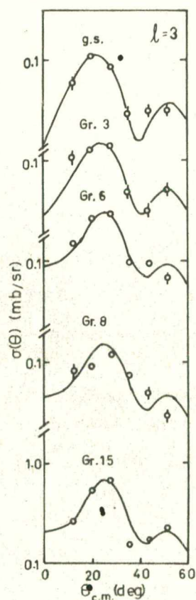
Fig. 3. Measured angular distributions fitted with l = 3 DWBA curves.
