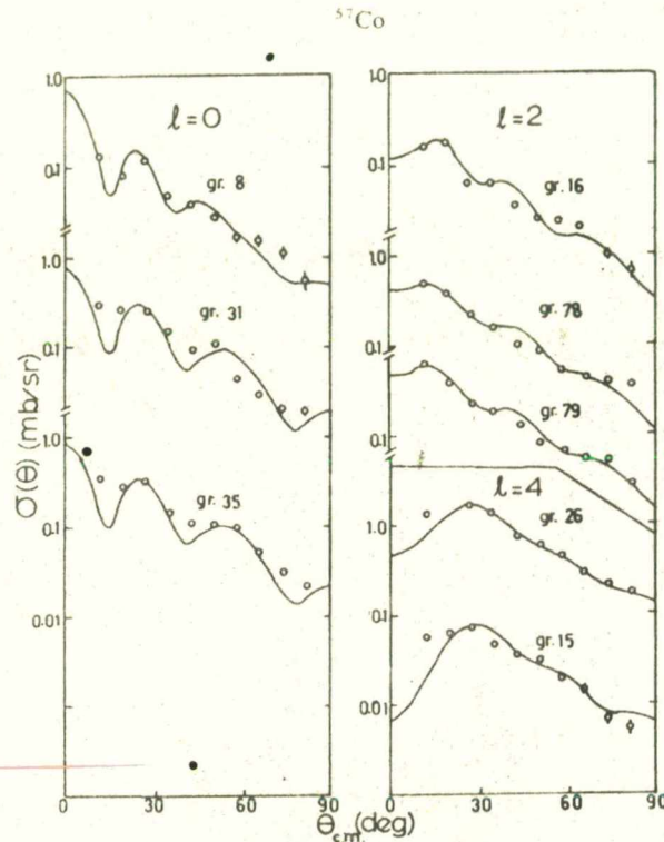
Fig. 4. Measured angular distributions fitted with l = 0, 2 and 4 DWBA curves.
