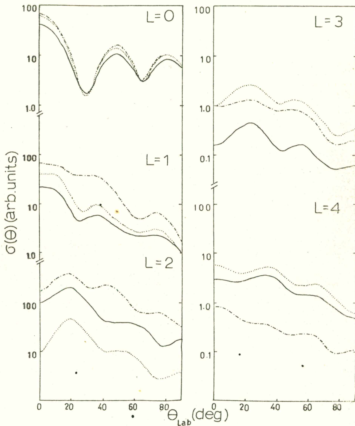
FIG. 7.3. DWBA curves with different potential parameters.
