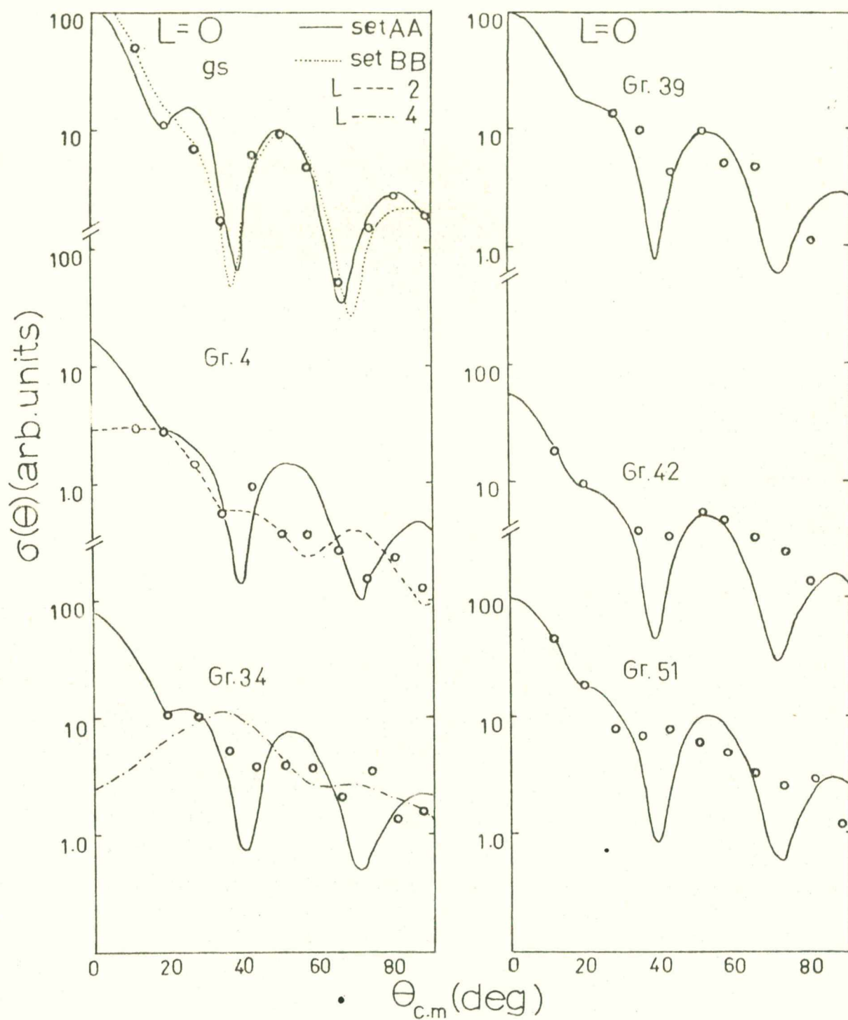
FIG.6.3. Experimental angular distributions fitted to L = 0 DWBA calculation.
