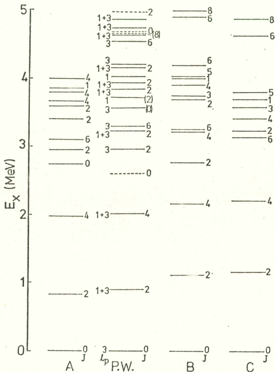
FIG. 5.9. Experimental level spectrum of ^{46}\text{Ti} compared with theory (Only positive-parity levels shown). P.W.: Present work [levels with l_p=3 character are shown by solid lines and other positive-parity levels are shown by broken lines; the J -values are from refs. Le 78, Au 78, Dr 78]. A: (Sk 75), B: (Pr 69), C: (Ku 78).
