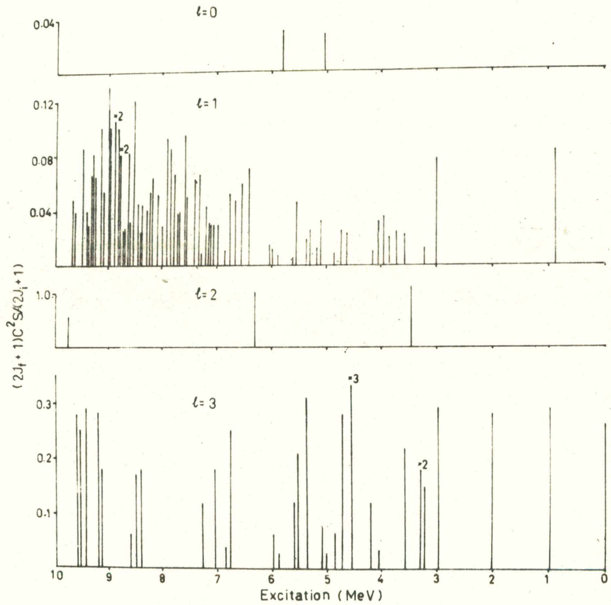
FIG. 5.8. The spectral distributions of single-particle strengths.
