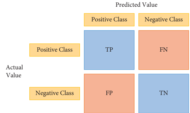
FIGURE 11: Confusion matrix.
