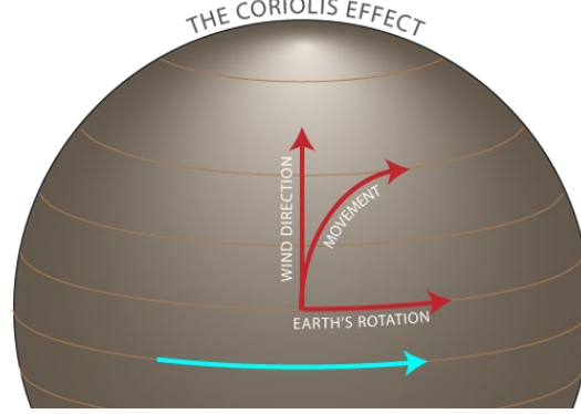
Figure 1.g: Coriolis Effect
