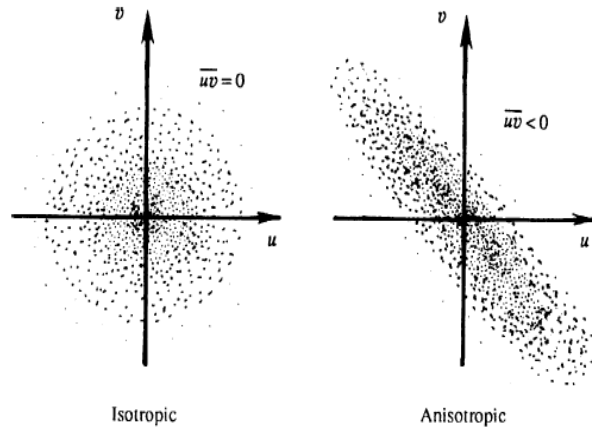
Figure 1.c: Isotropic Turbulence
