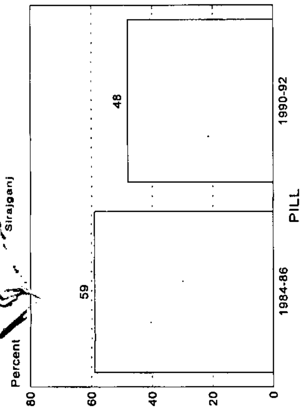
Figure 6: Contraception Rate by Method, Area and Year
