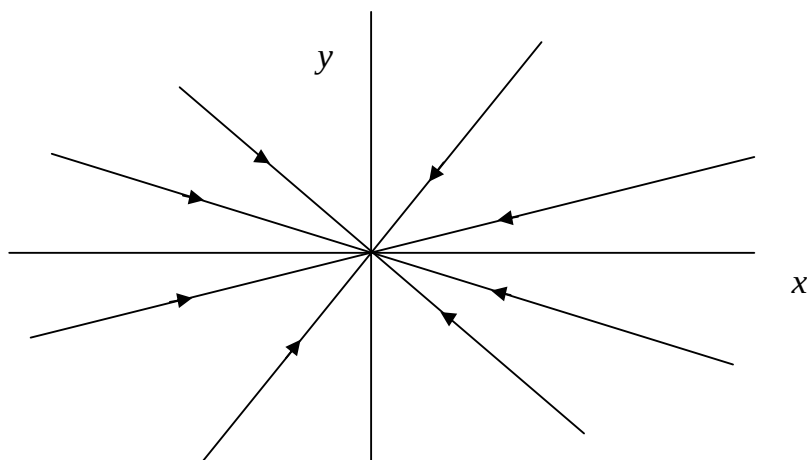
Figure 2.5.6: Star singularity
