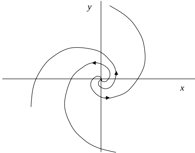
Figure 2.5.3: Spiral singularity
