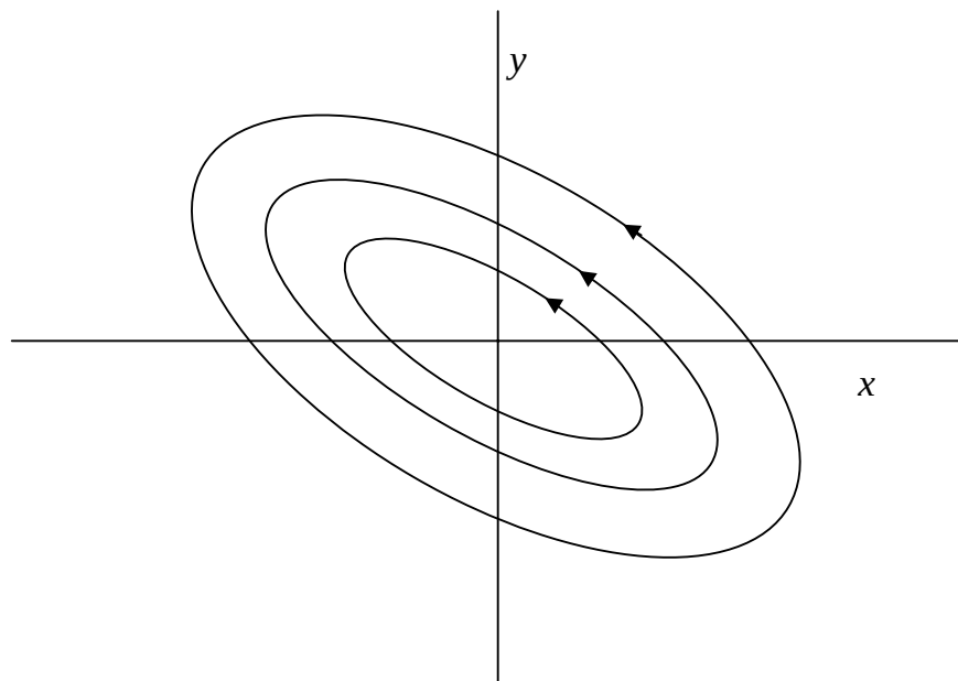
Figure 2.5.4: Centre singularity
